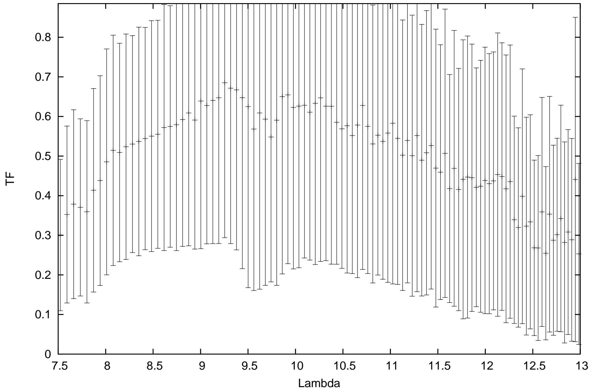
calHIP90496_flux0.238088_diam3.99_r.MIDI.2013-04-23T06_37_20.000_D0G1
