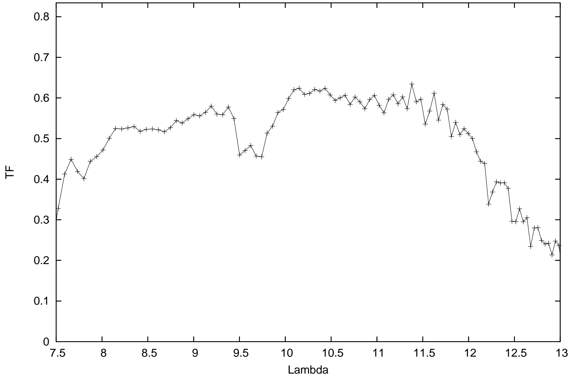
calHIP86742_flux0.007006_diam4.37_r.MIDI.2013-04-23T05_35_42.000_H011
