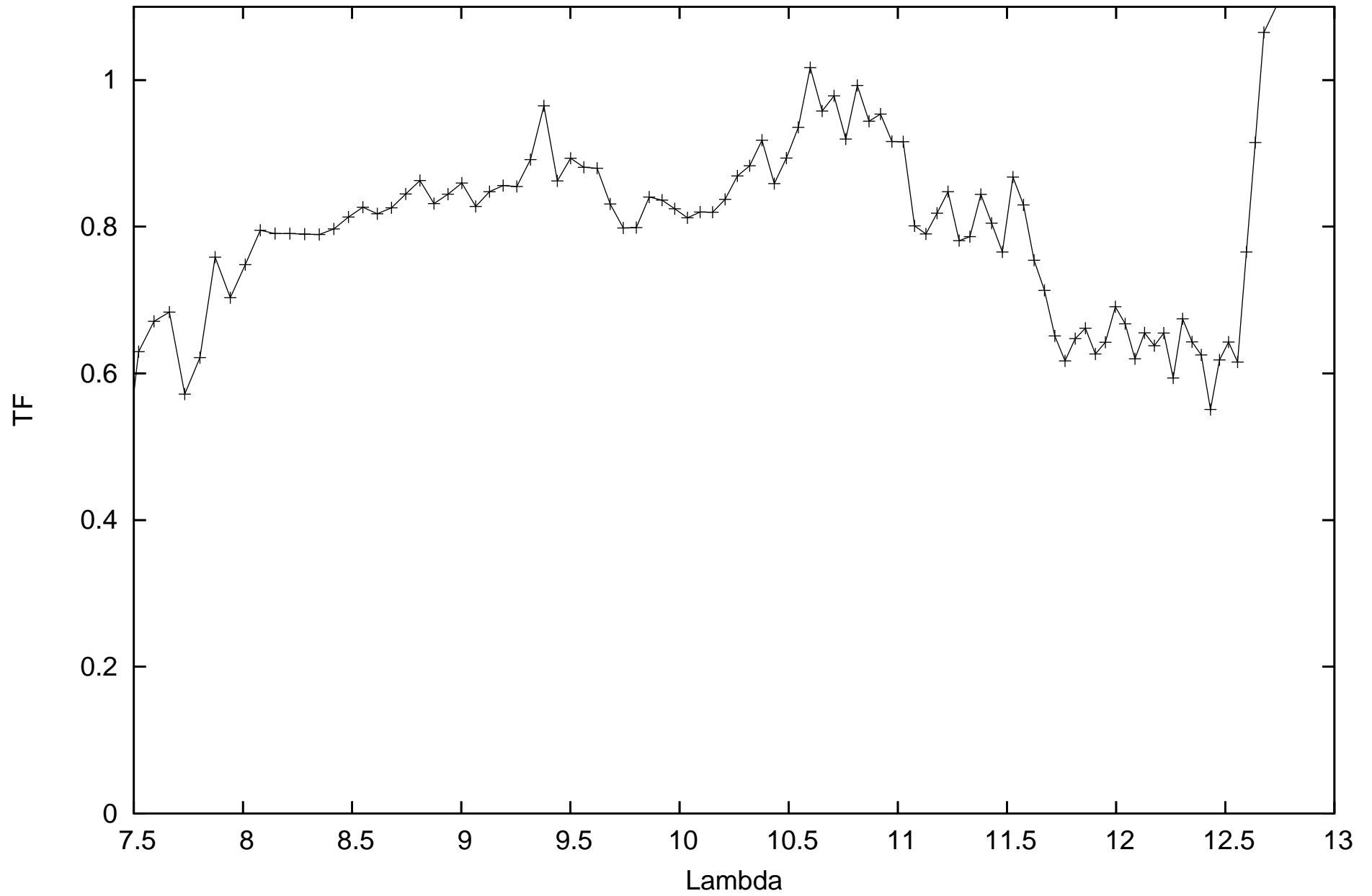
calHD125687_flux0.4_diam4.03_r.MIDI.2013-04-18T06_11_13.000_D0B2
