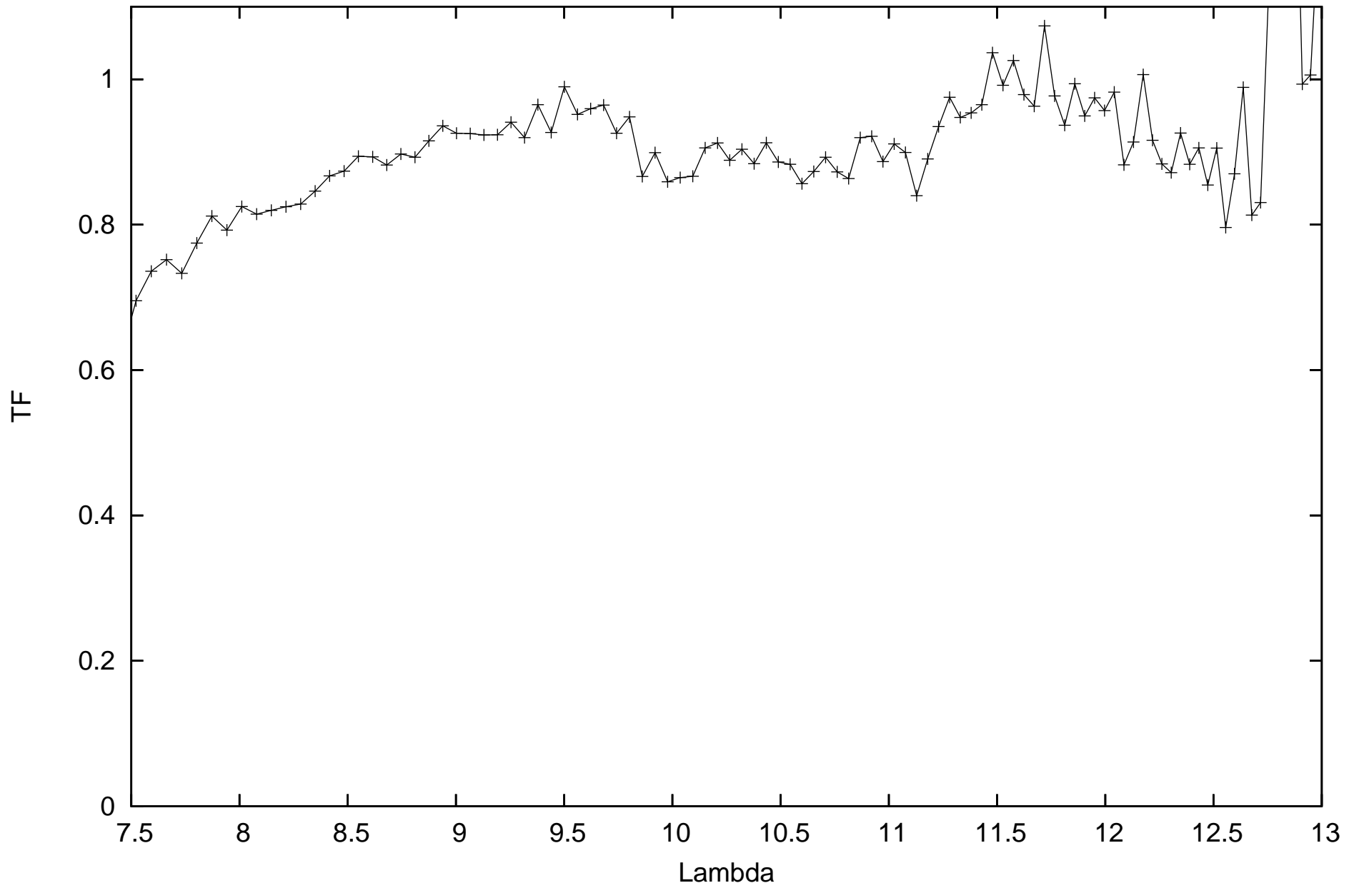
calHD107446_flux0.22_diam4.43_r.MIDI.2013-04-17T02_19_26.000_B2A1
