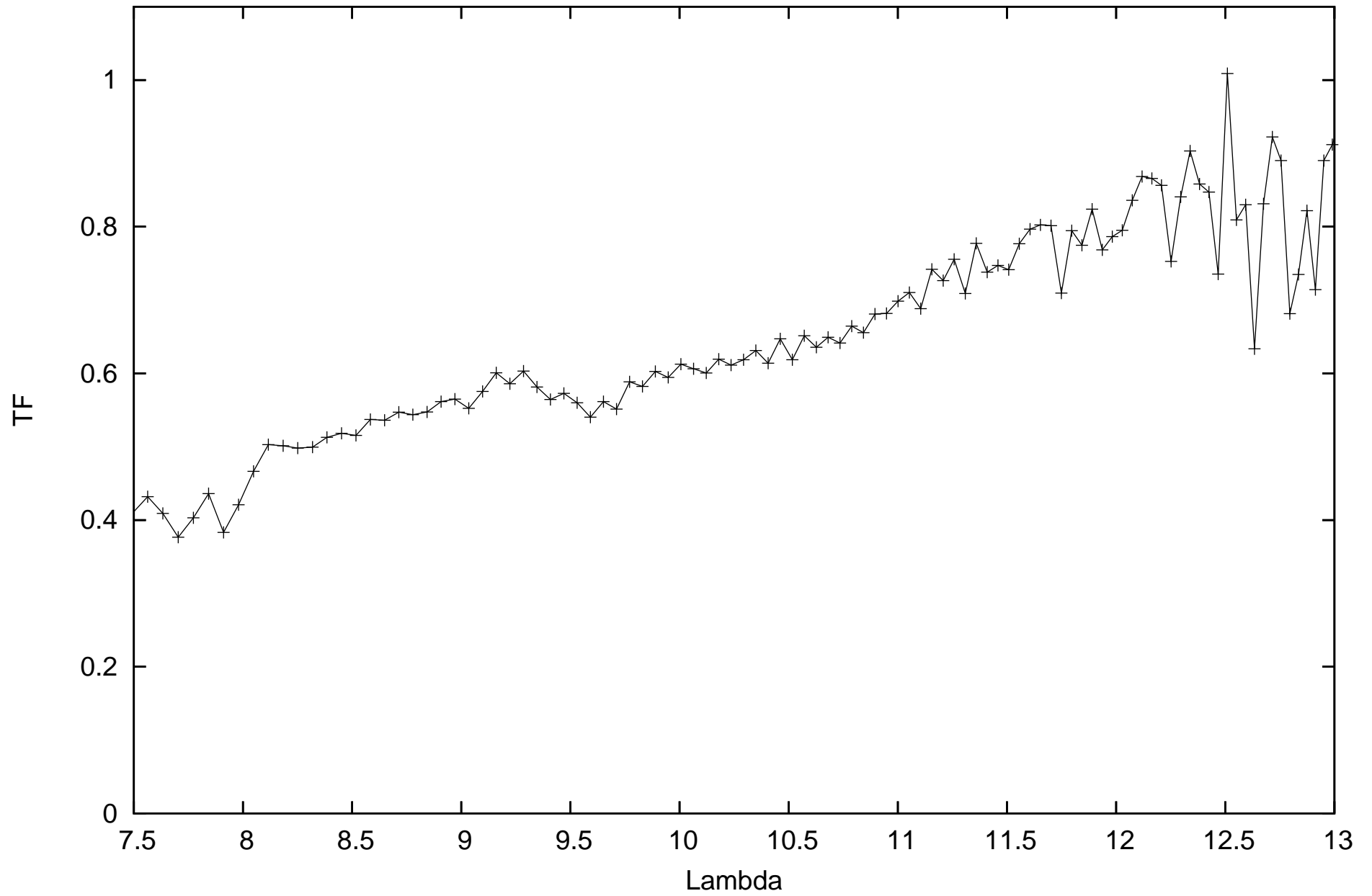
calHD81797_flux-1.49_diam9.14_r.MIDI.2013-04-12T03_43_59.112_D0B2
