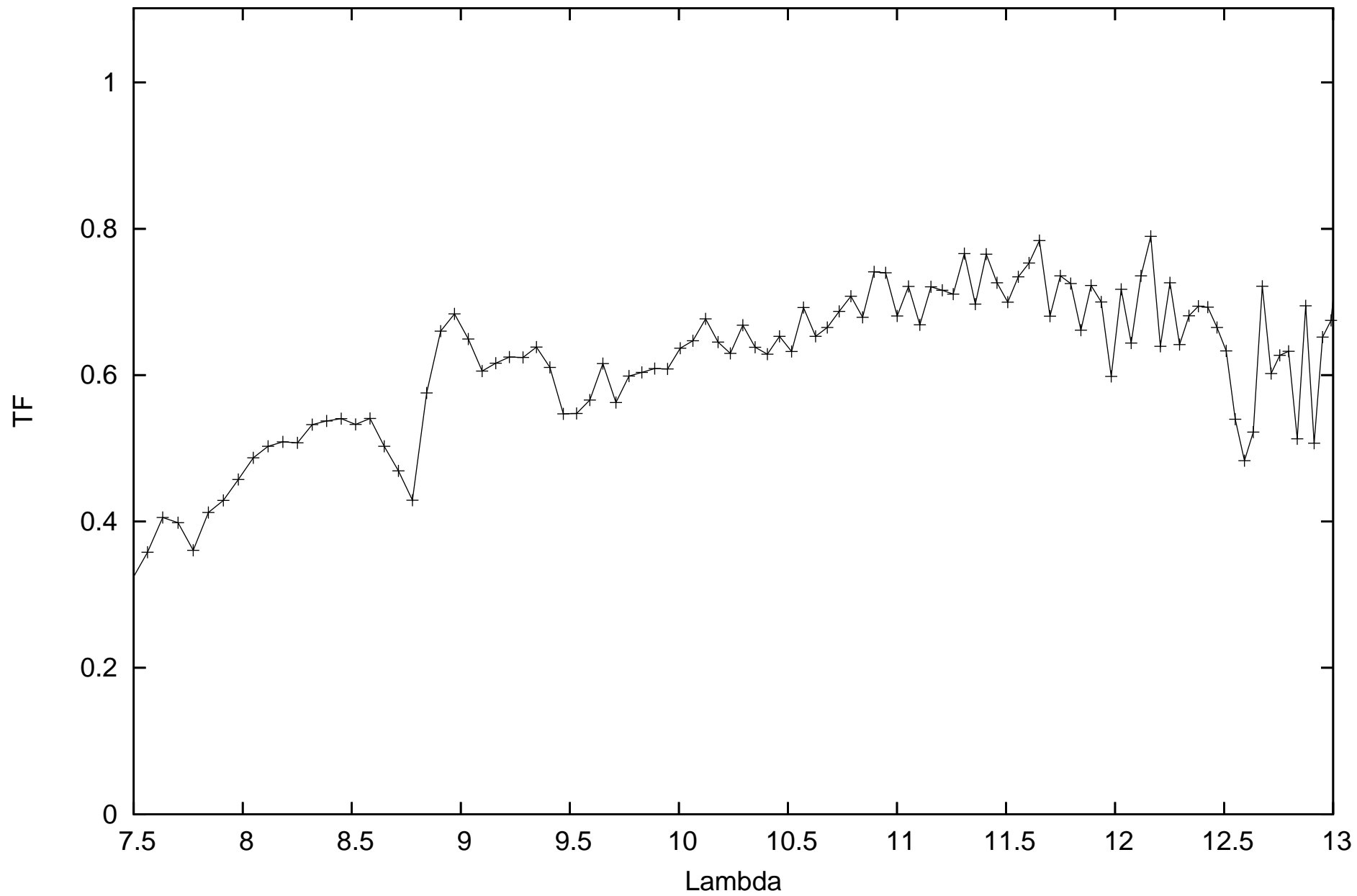
calHIP83081_flux-0.81238_diam6.88_r.MIDI.2013-04-09T10_06_34.932_G111
