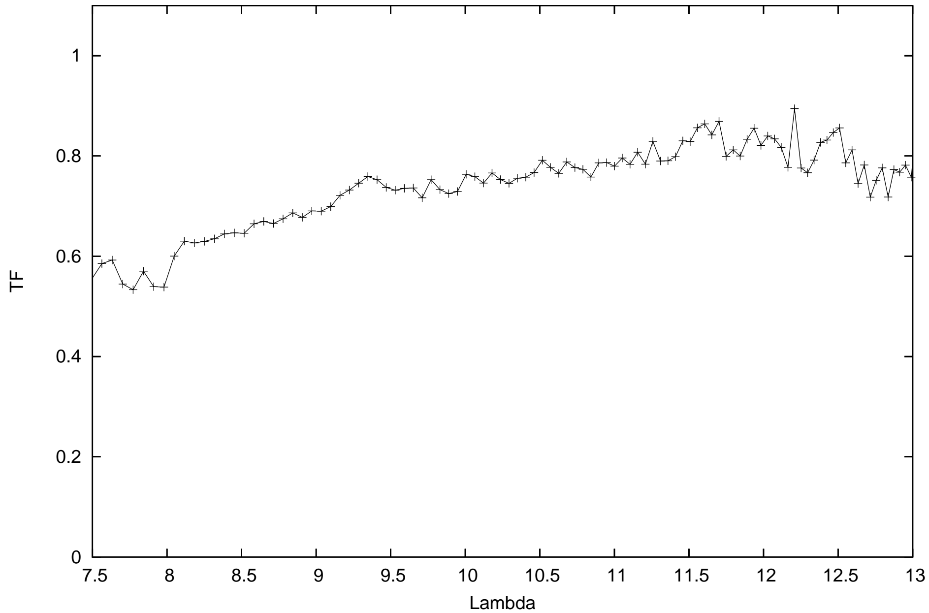
calHIP73714_flux-1.78451_diam11.15_r.MIDI.2013-04-07T05_16_09.112_D0H0
