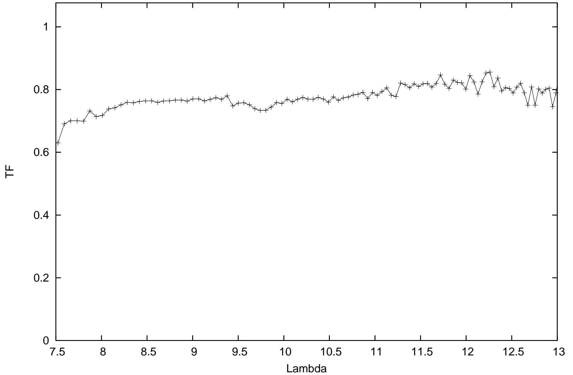
calHD81797_flux-1.49_diam9.14_r.MIDI.2013-03-28T03_50_21.000_C1B2
