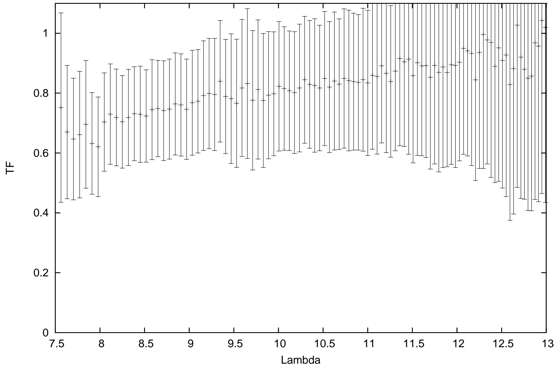
calHD48915_flux-1.39_diam6.09_r.MIDI.2013-03-06T02_39_25.112_G211
