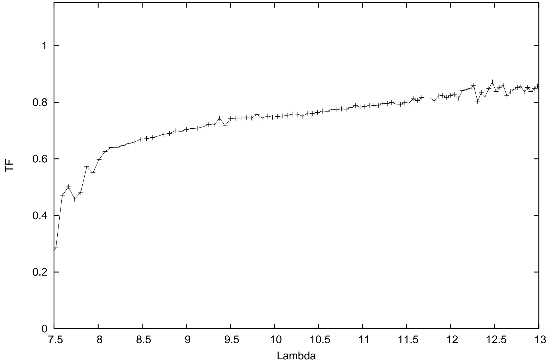
calHD98292_flux0.92_diam3.35_r.MIDI.2013-03-04T07_26_35.000_U1U4
