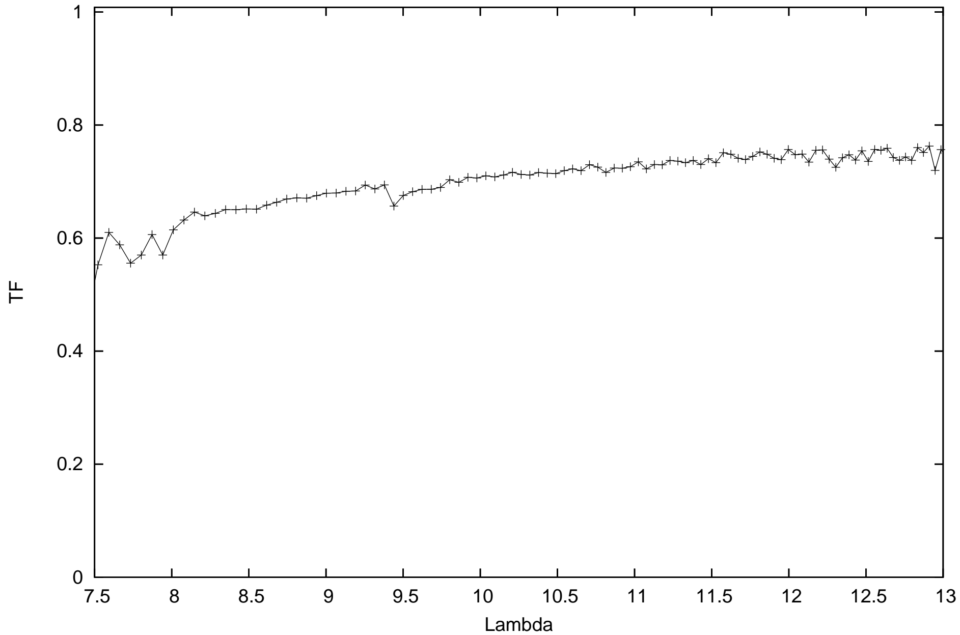
calHD98292_flux0.92_diam3.35_r.MIDI.2013-03-01T07_05_13.000_U3U4
