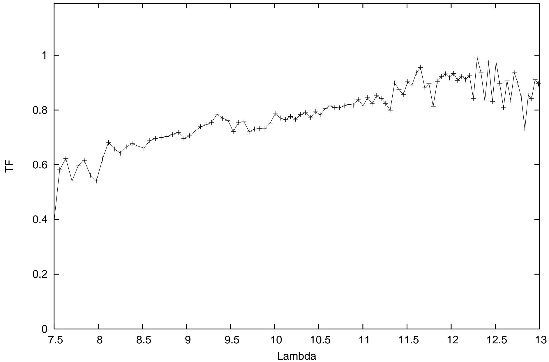
calHD81797_flux-1.49_diam9.14_r.MIDI.2013-02-14T05_23_27.113_D0G1
