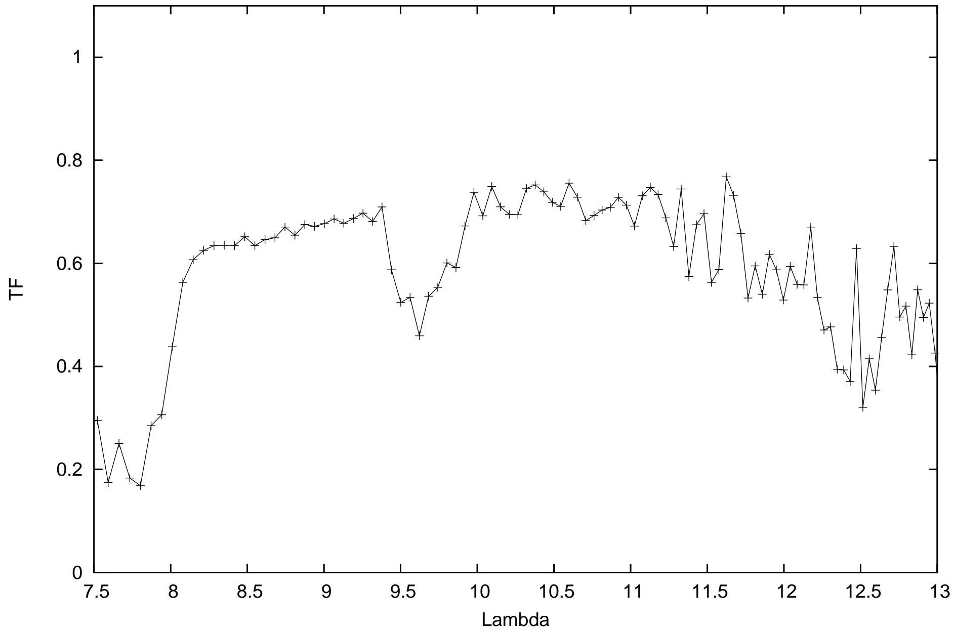
calHD107446_flux0.22_diam4.43_r.MIDI.2012-03-29T02_29_10.000_I1A1
