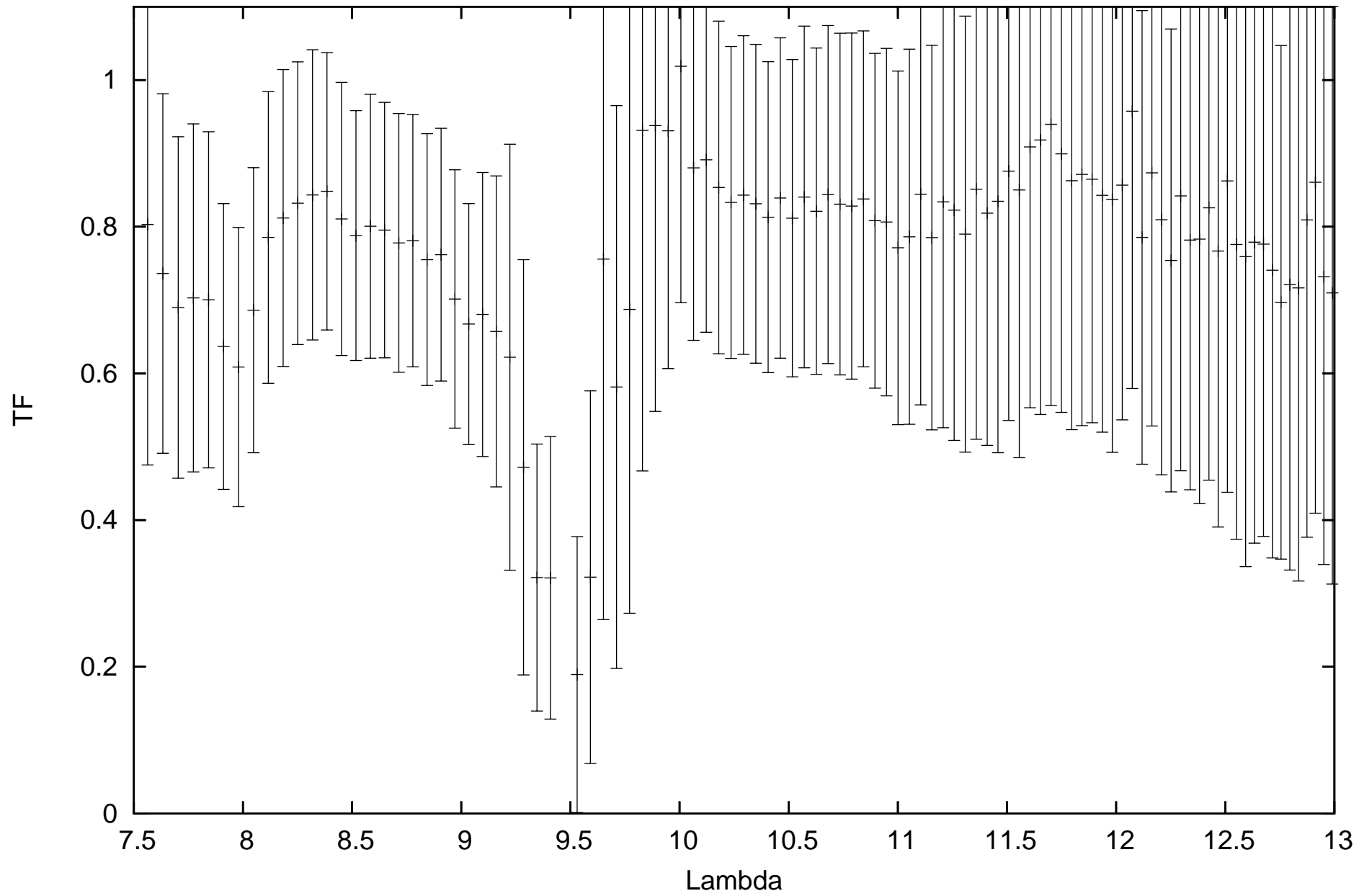
calHD48915_flux-1.39_diam6.09_r.MIDI.2012-12-11T03_28_40.113_C1A1
