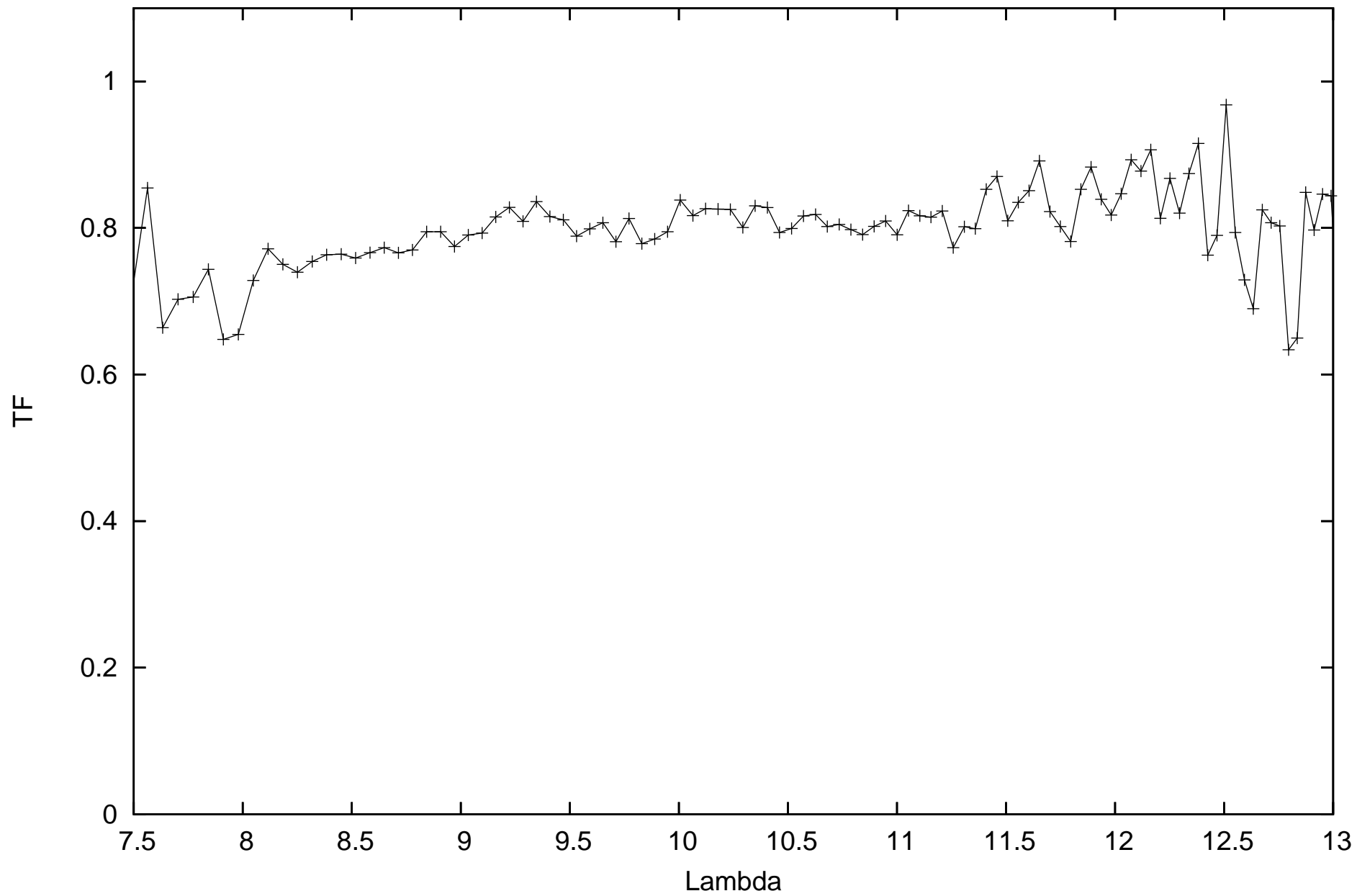
calHD48915_flux-1.39_diam6.09_r.MIDI.2012-12-10T05_06_17.112_B2A1
