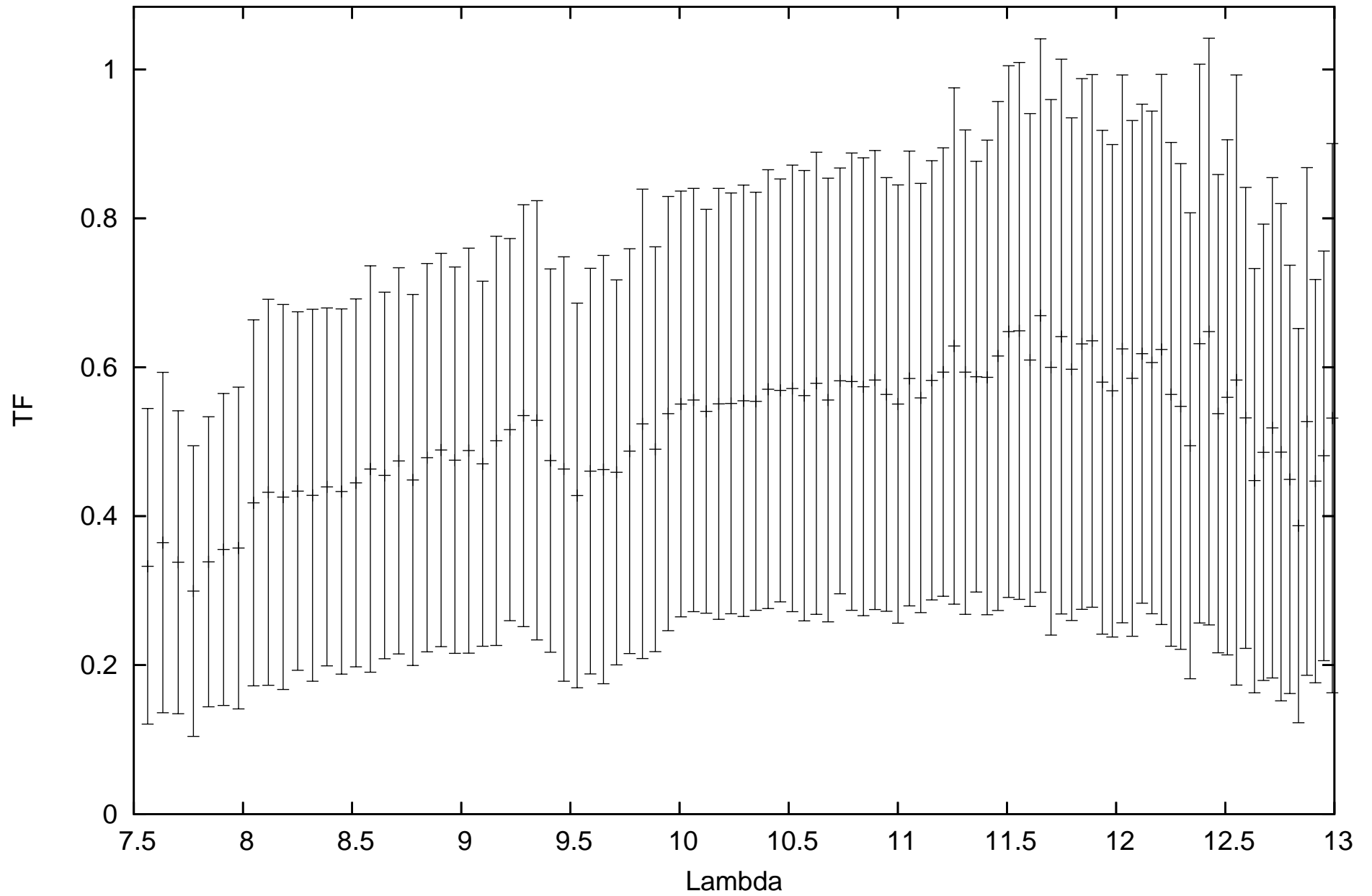
calHD206778_flux-1.04_diam7.59_r.MIDI.2012-10-25T03_23_14.135_H011
