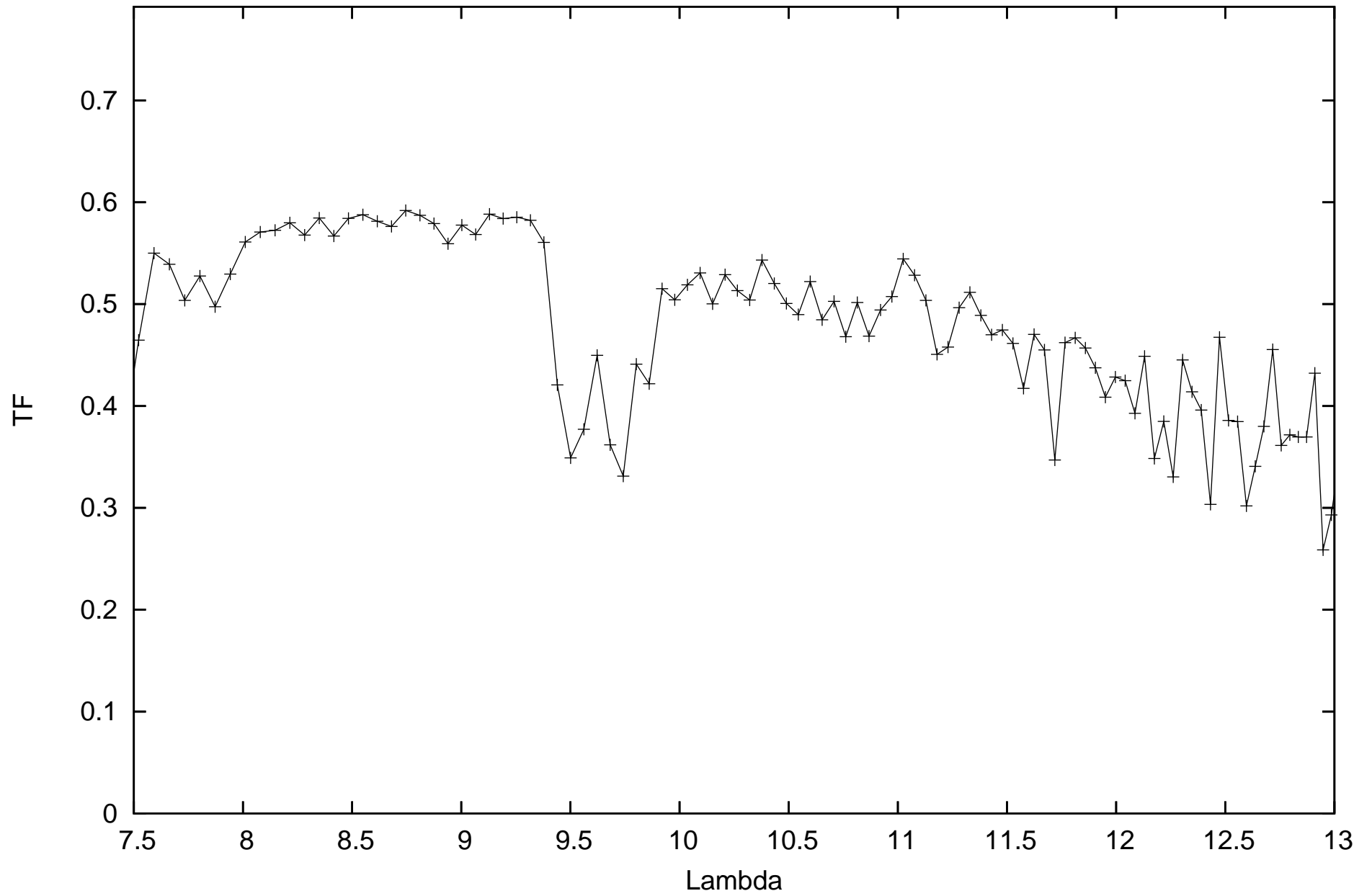
calHIP90496_flux0.238088_diam3.99_r.MIDI.2012-10-20T00_50_28.000_C1A1
