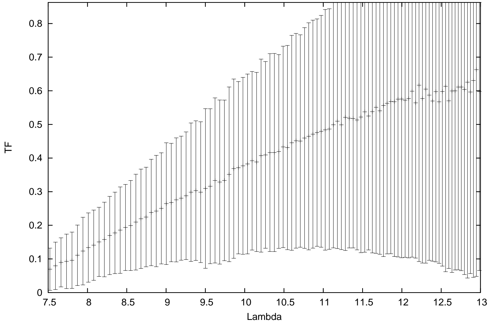
calHIP14135_flux-1.95419_diam12.27_r.MIDI.2012-10-03T07_50_49.000_K0A1
