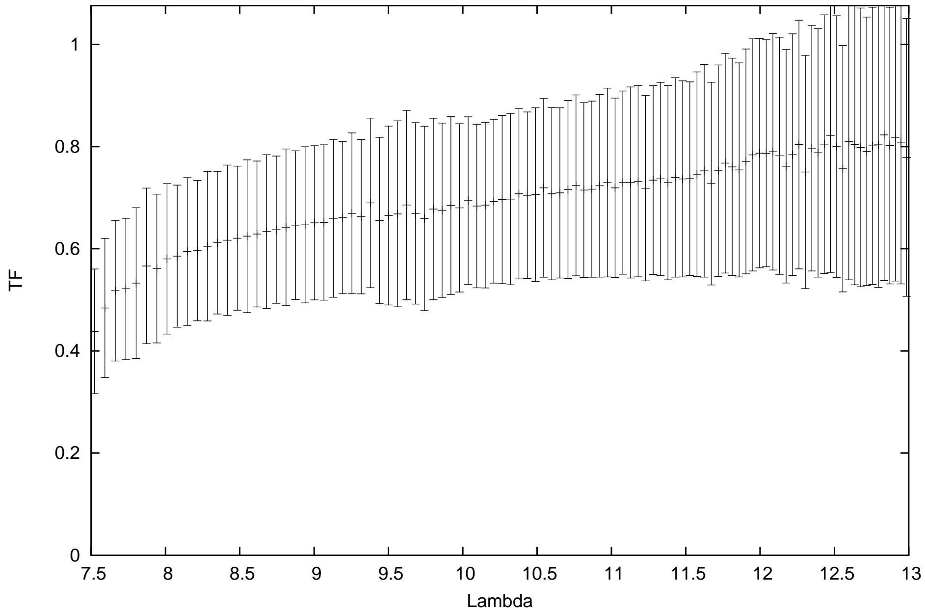
calHD167618_flux-1.82_diam11.66_r.MIDI.2012-09-30T01_43_14.000_H0G1
