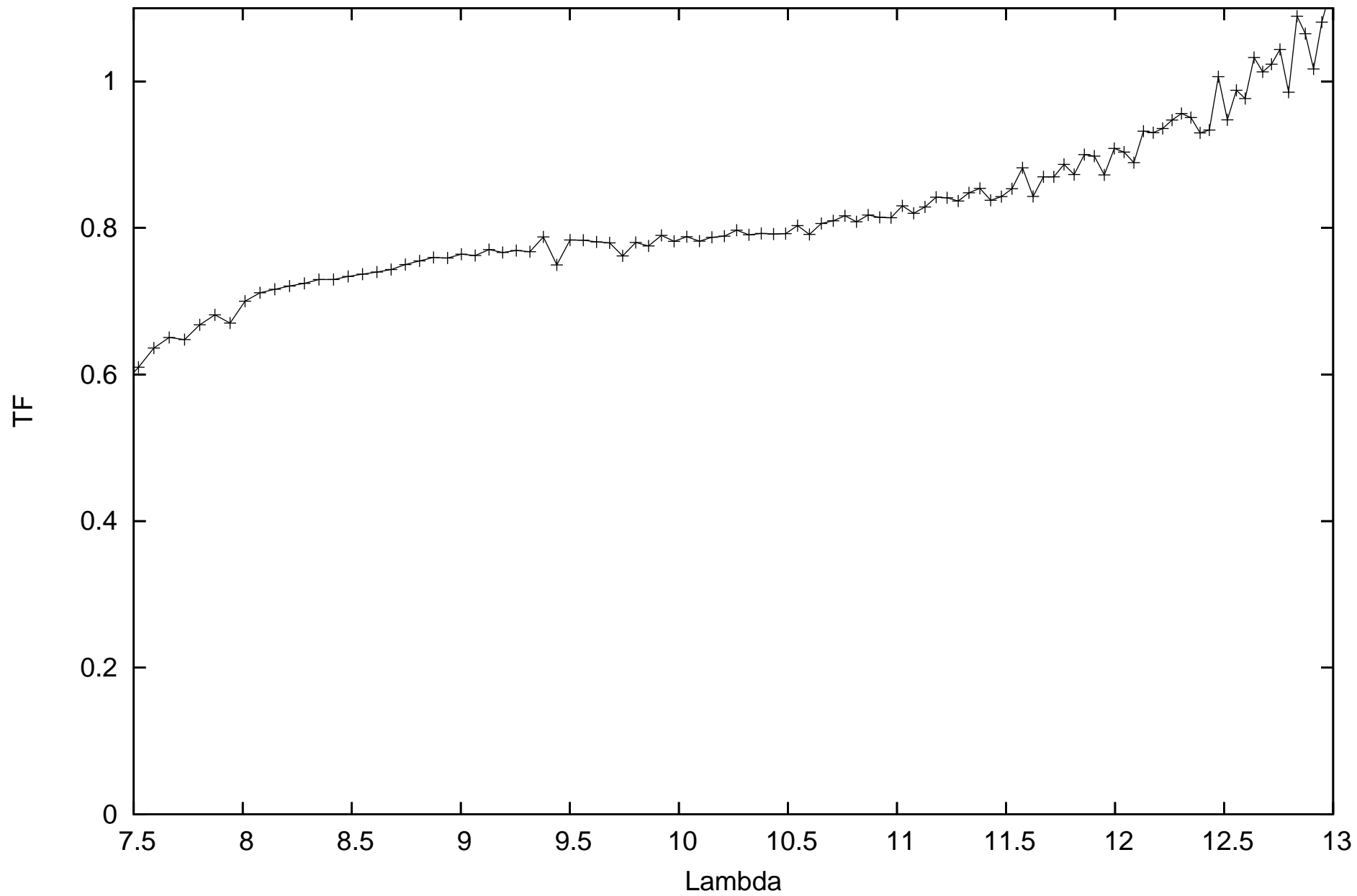
calHD167618_flux-1.82_diam11.66_r.MIDI.2012-09-24T23_42_02.000_D0C1
