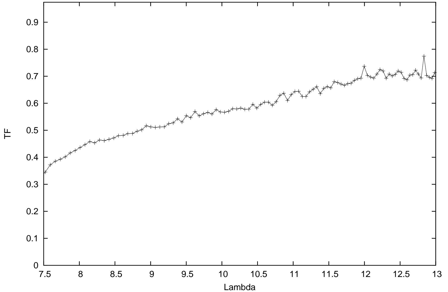
calHD167618_flux-1.82_diam11.66_r.MIDI.2012-09-24T00_31_55.000_D0B2
