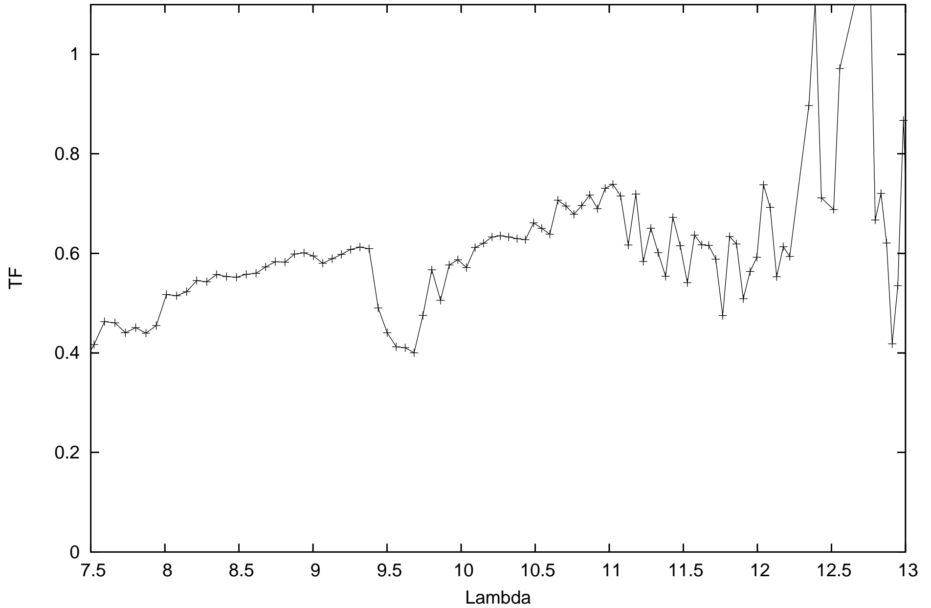
calHD107446_flux0.22_diam4.43_r.MIDI.2012-07-22T23_26_20.000_B2A1
