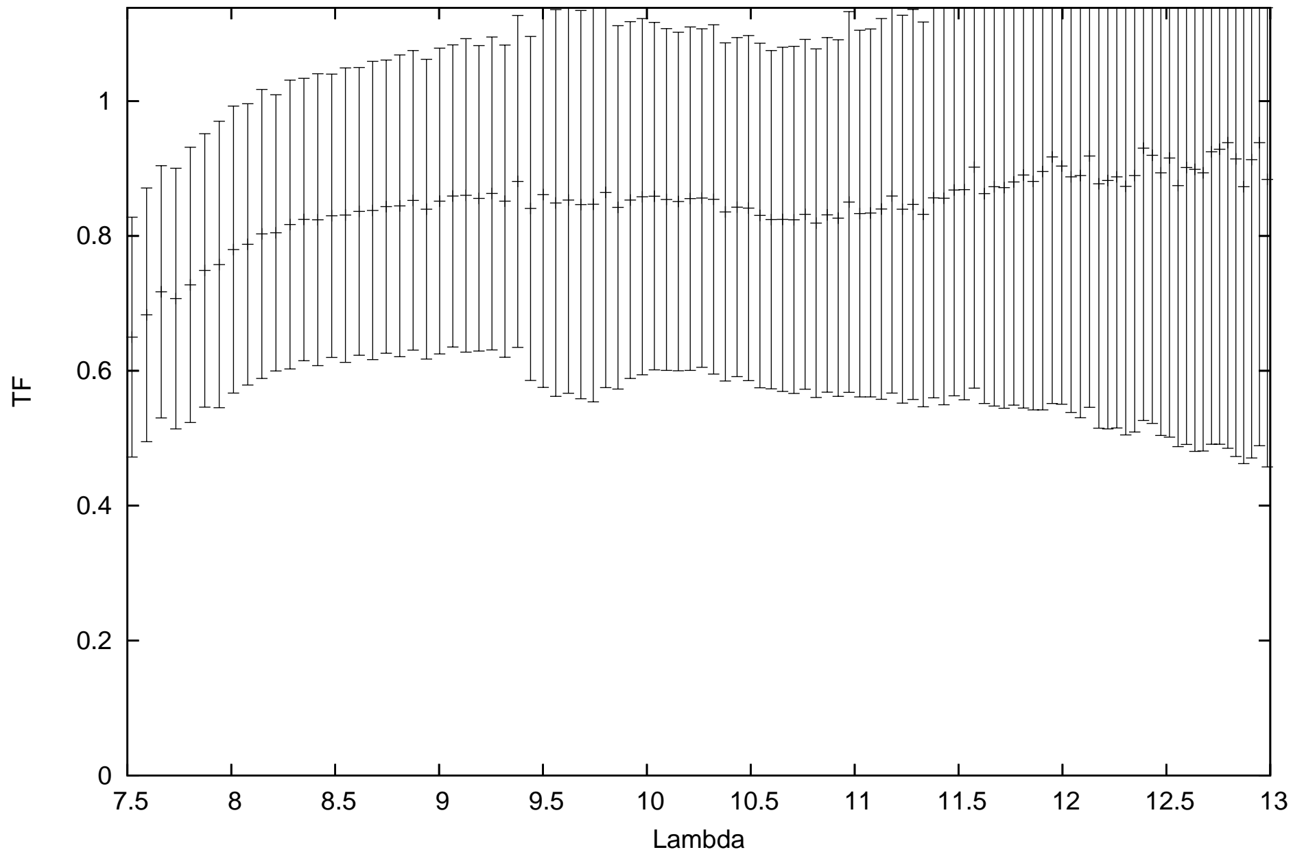
calHD167618_flux-1.82_diam11.66_r.MIDI.2012-07-22T02_01_07.000_D0B2
