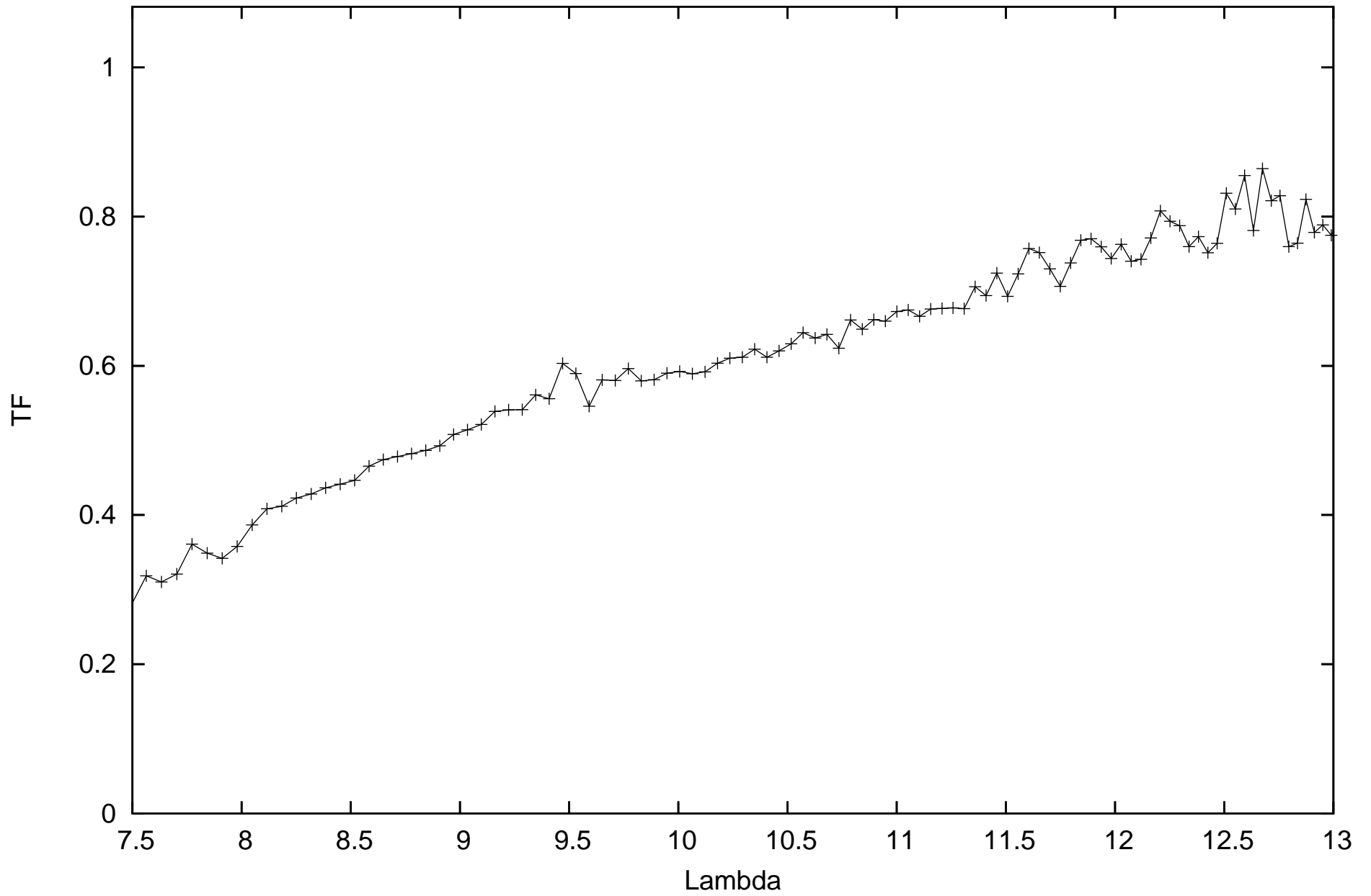
calHD167618_flux-1.82_diam11.66_r.MIDI.2012-06-16T04_51_38.112_D011
