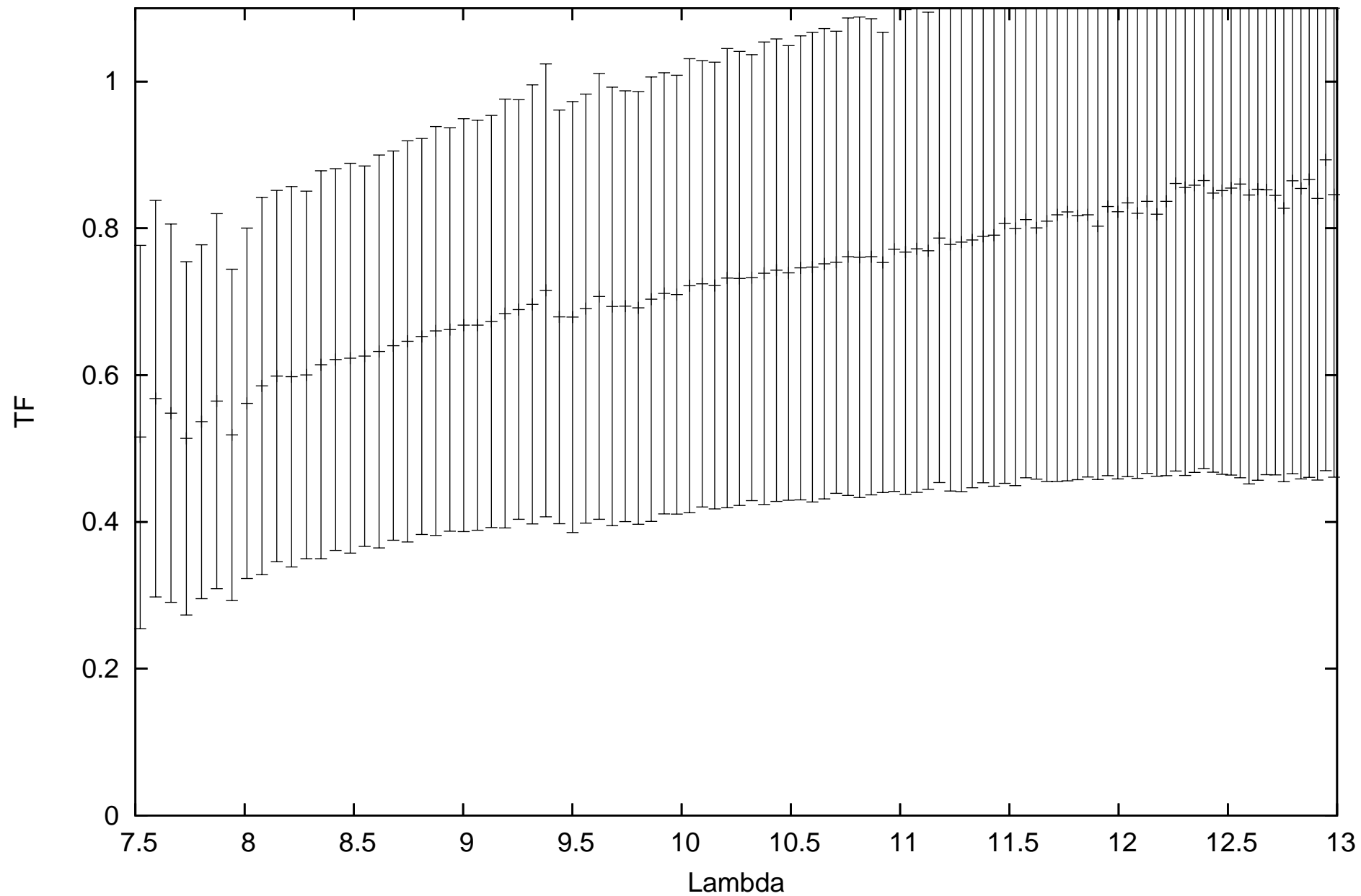
calHIP55219_flux0.091804_diam4.49_r.MIDI.2012-06-01T23_35_36.000_U2U3
