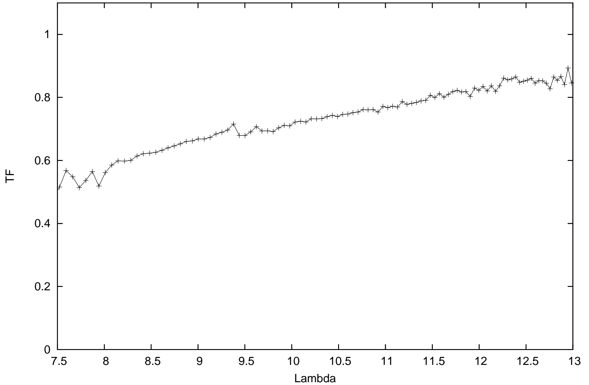
calHIP55219_flux0.091804_diam4.49_r.MIDI.2012-06-01T23_35_36.000_U2U3
