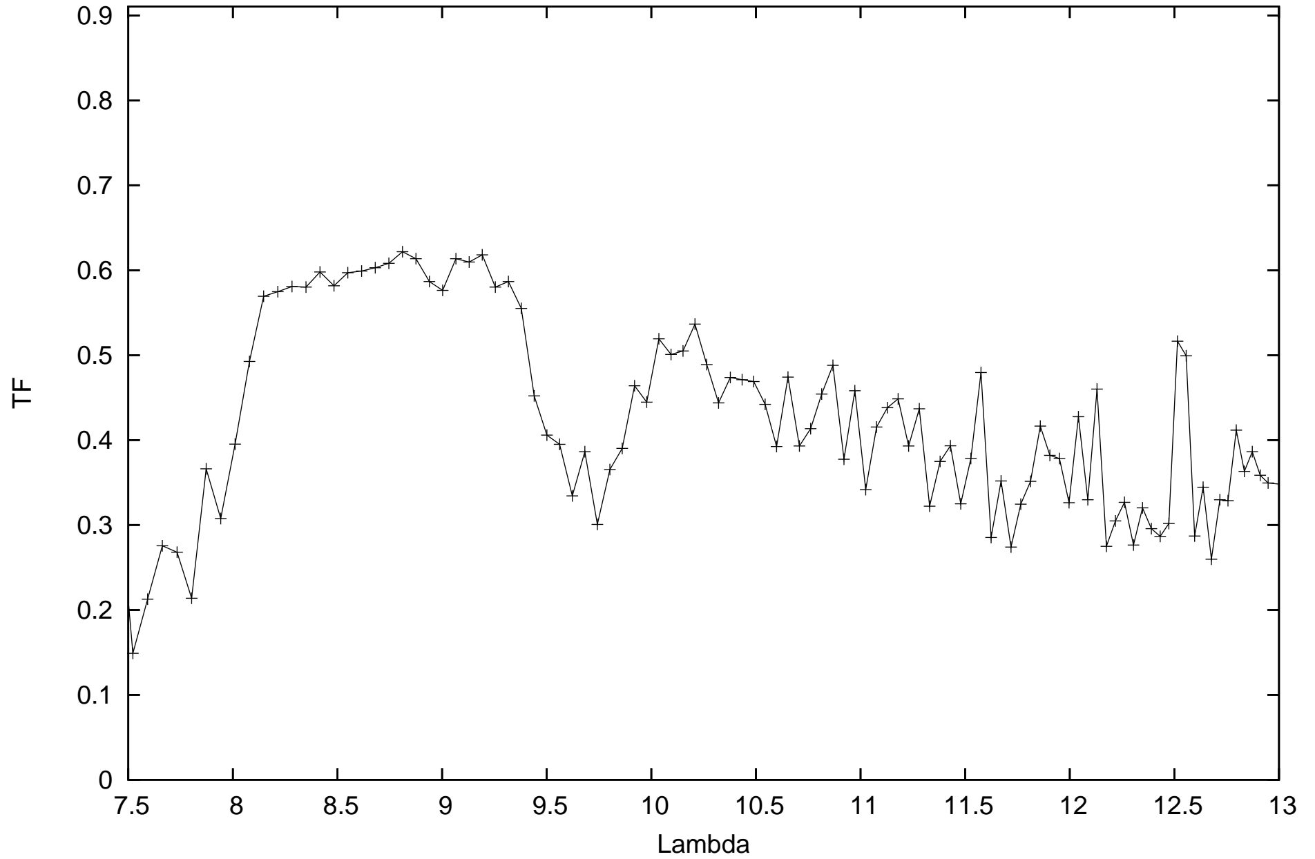
calHIP78870_flux3.70545_diam0.82654_r.MIDI.2012-05-10T07_33_20.000_U1U3
