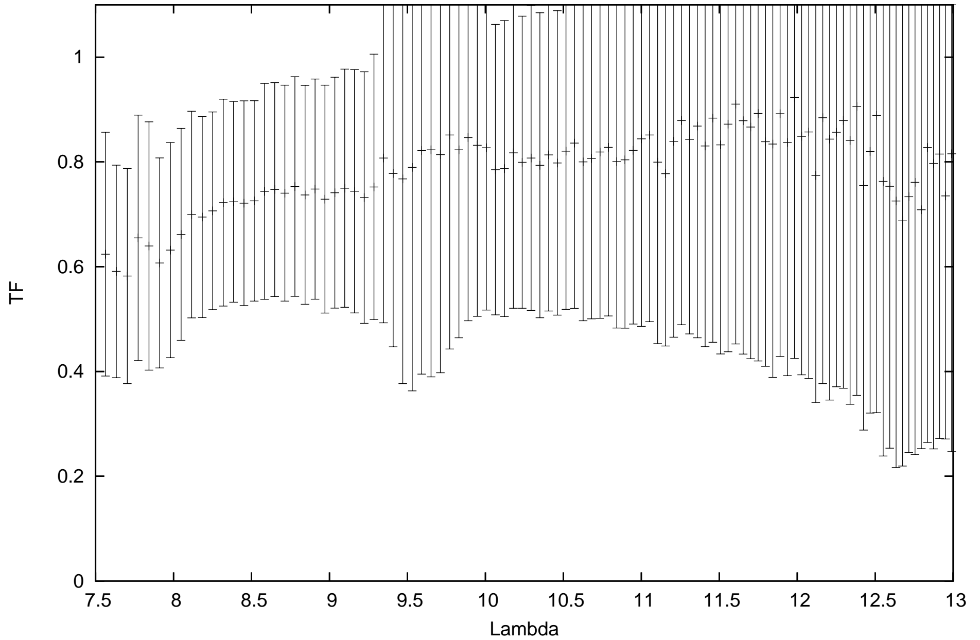
calHD81797_flux-1.49_diam9.14_r.MIDI.2012-05-01T00_43_49.293_C1B2
