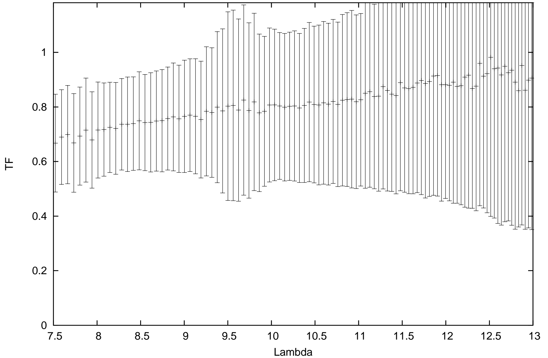
calHD81797_flux-1.49_diam9.14_r.MIDI.2012-04-30T23_39_25.000_C1B2
