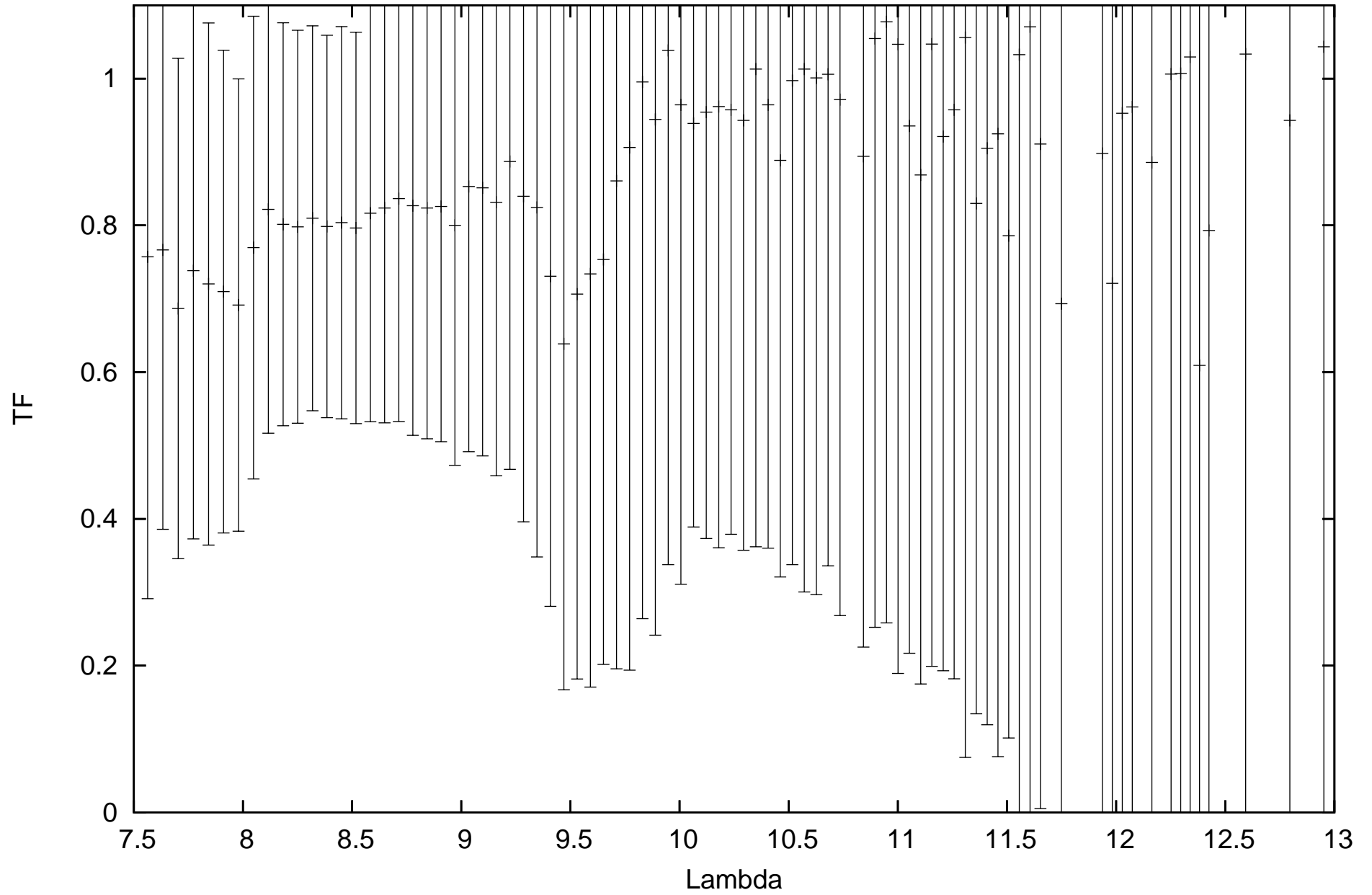
calHD123139_flux-0.39_diam5.34_r.MIDI.2012-05-01T03_03_26.293_B2A1
