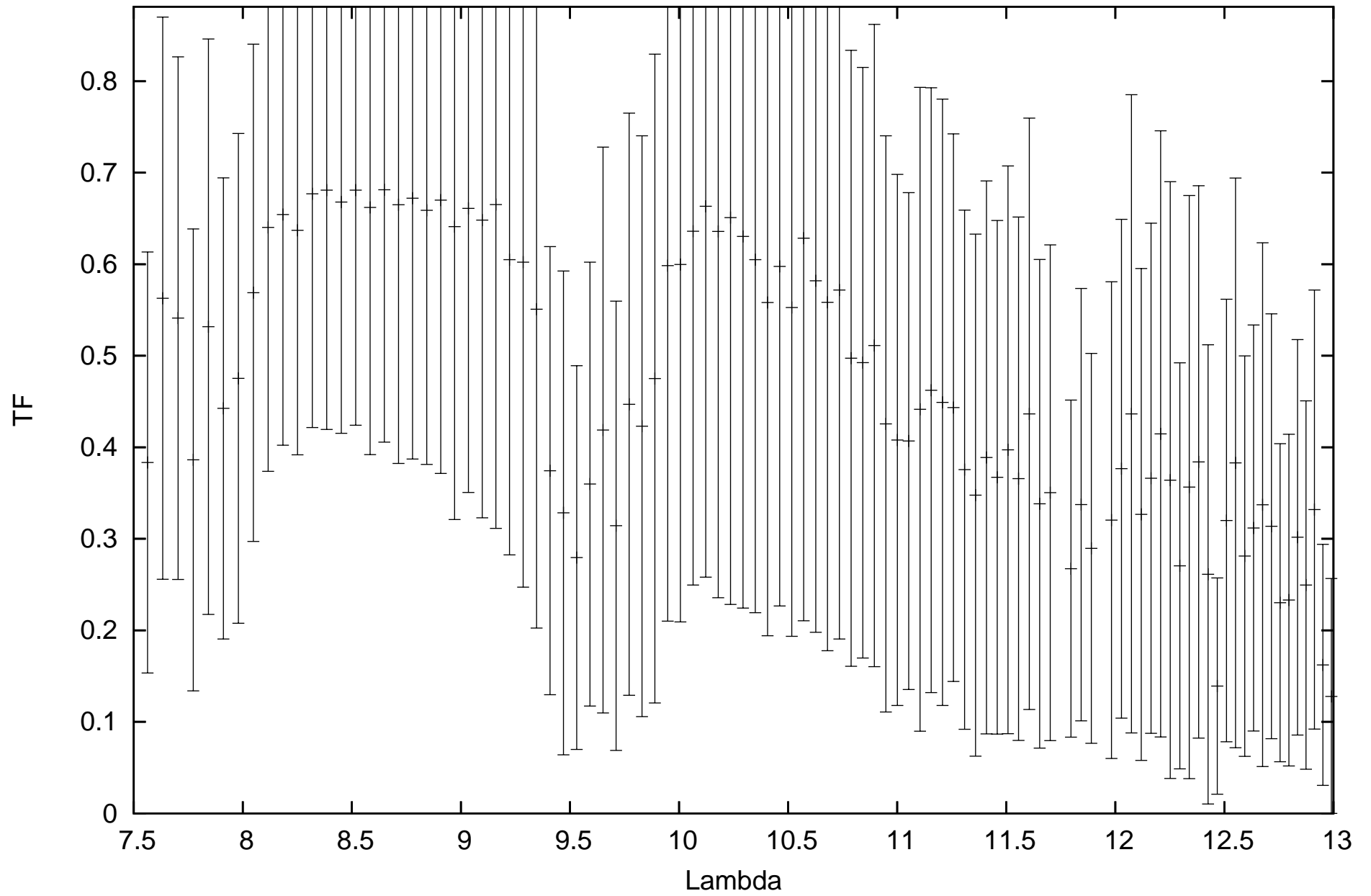
calHD112142_flux-0.18_diam5.44_r.MIDI.2012-05-01T03_26_56.293_B2A1
