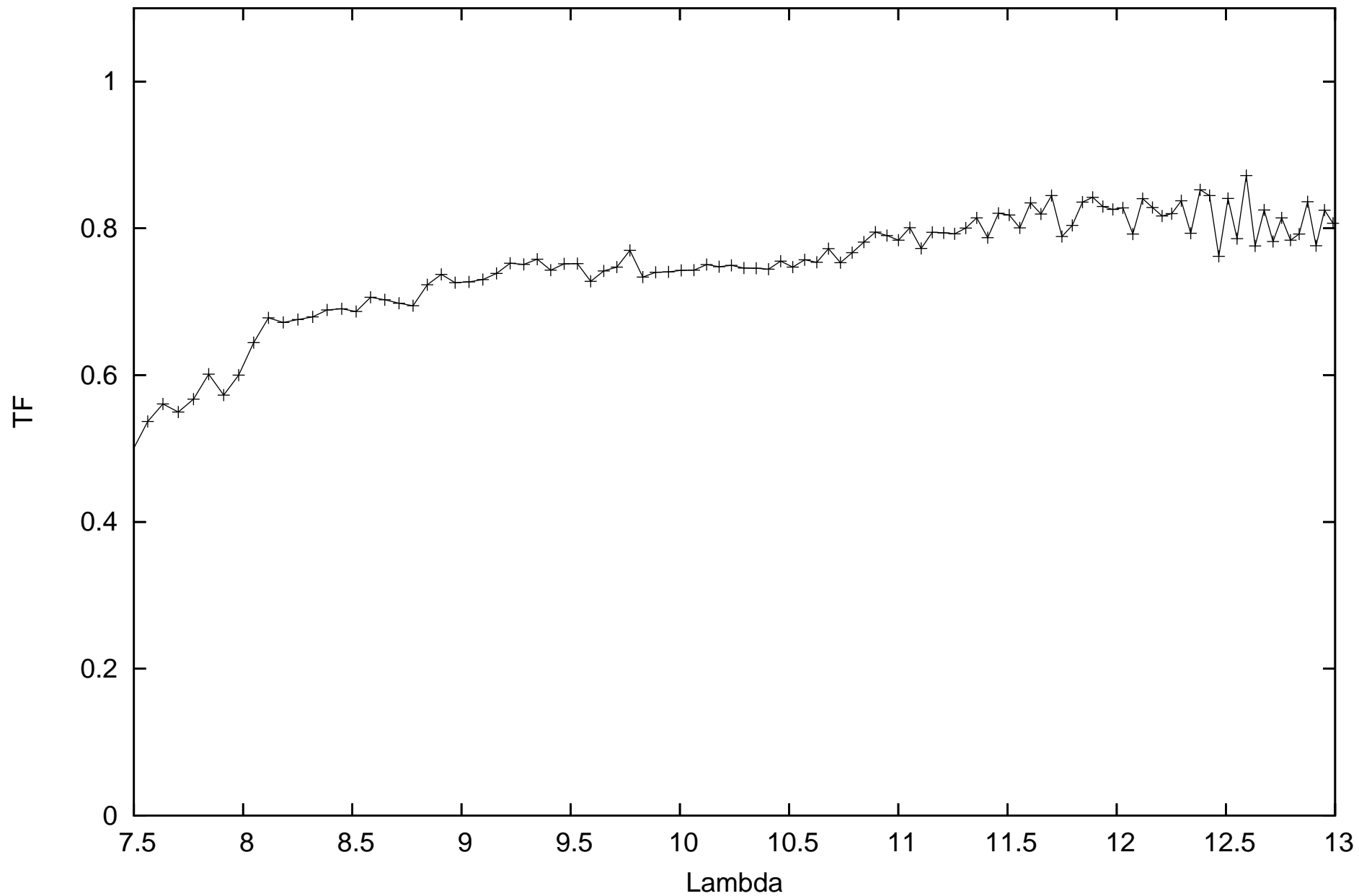
calHD152980_flux0.64_diam3.62_r.MIDI.2012-04-06T09_36_55.767_U1U2
