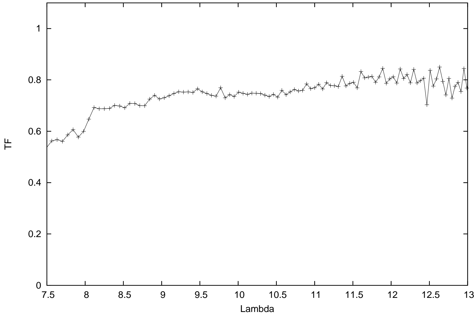
calHD152980_flux0.64_diam3.62_r.MIDI.2012-04-06T08_56_46.969_U1U2
