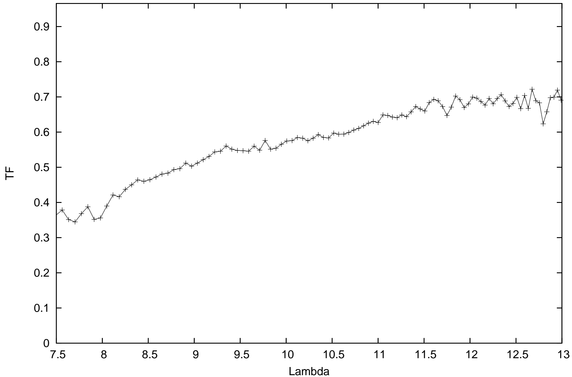
calHD152980_flux0.64_diam3.62_r.MIDI.2012-04-05T09_10_36.767_U2U3
