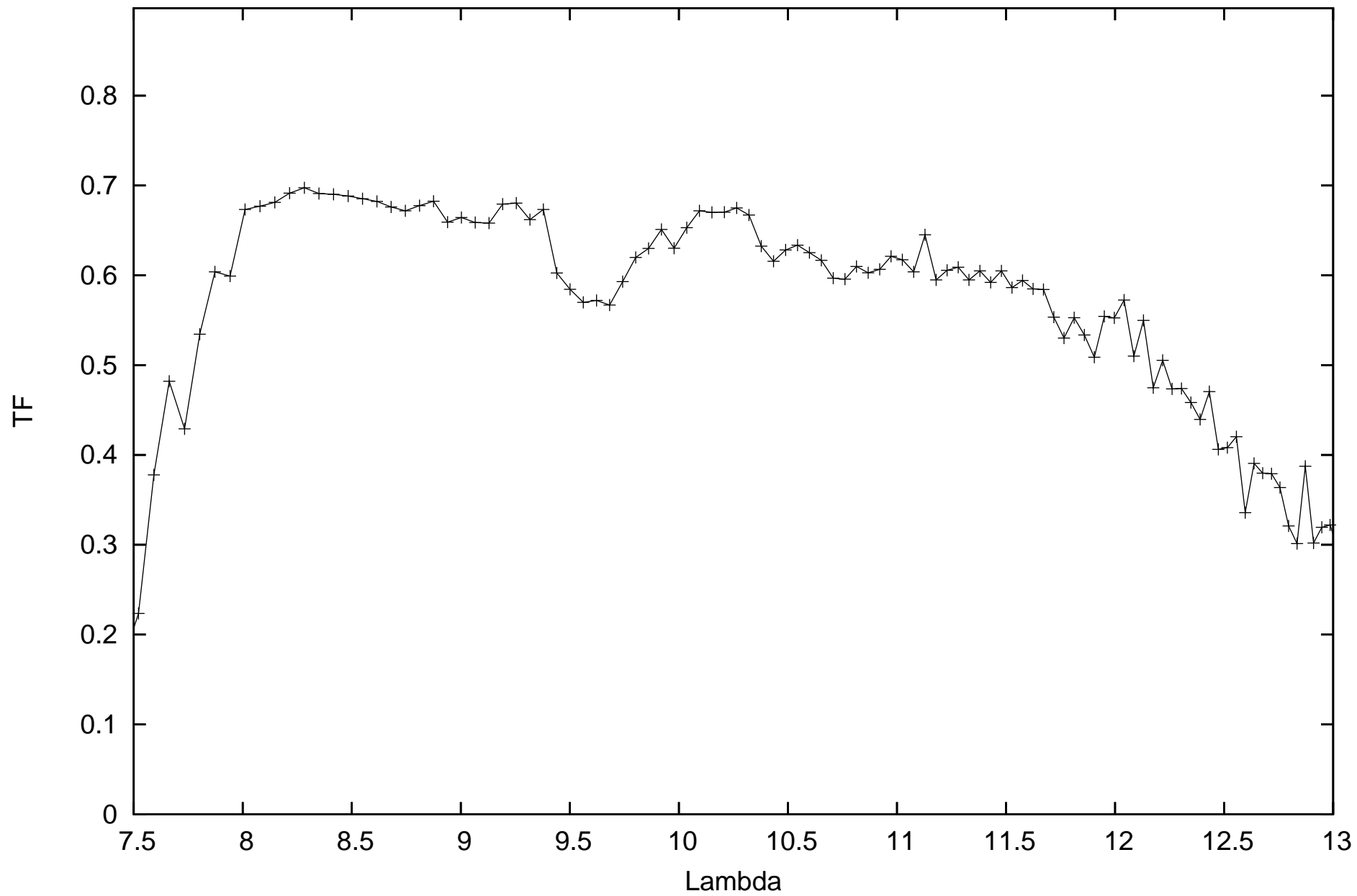
calHIP82363_flux-0.3207_diam5.52_r.MIDI.2012-04-01T09_23_35.000_G1K0
