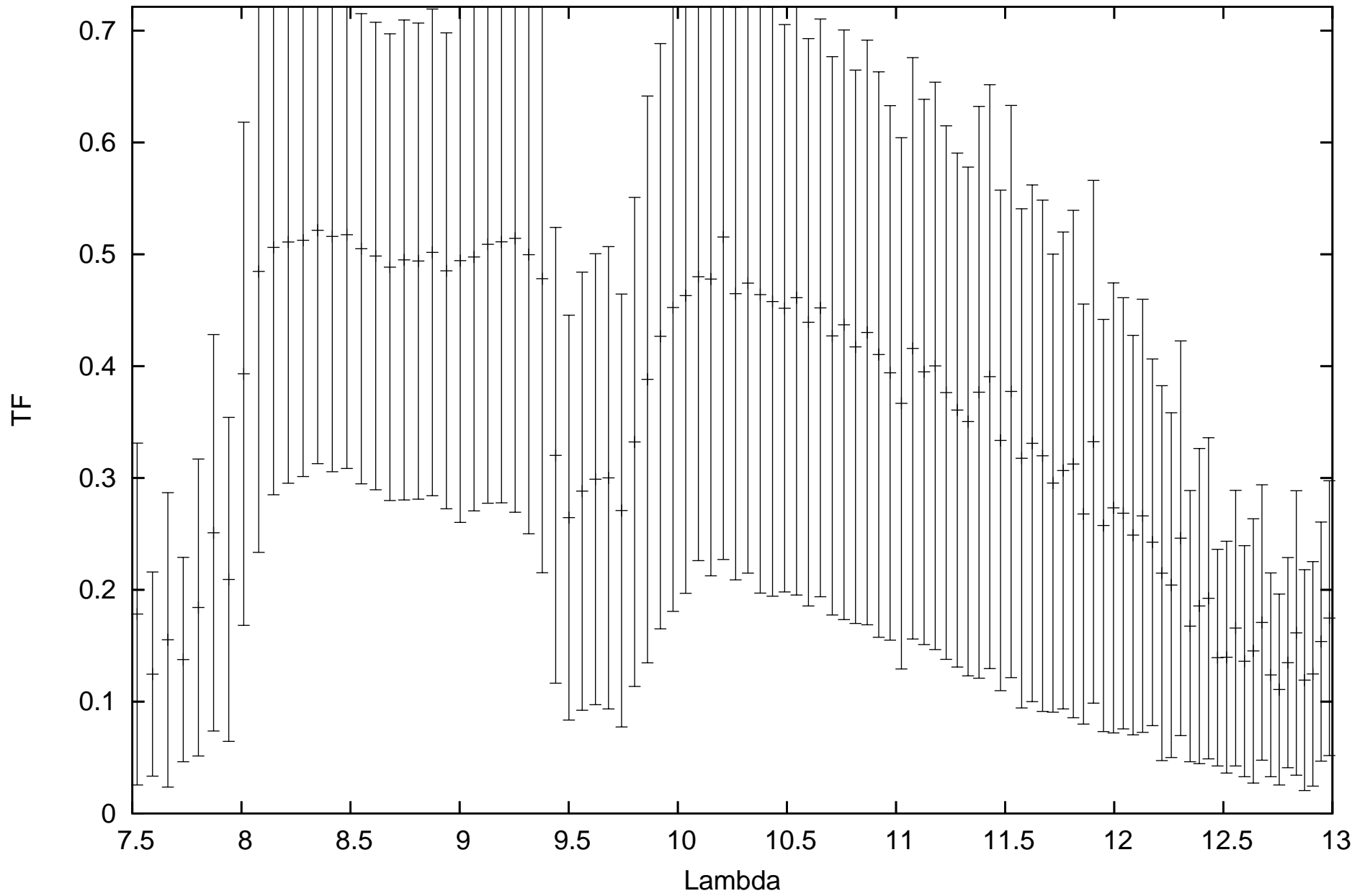
calHD107446_flux0.22_diam4.43_r.MIDI.2012-04-01T08_40_54.000_G1K0
