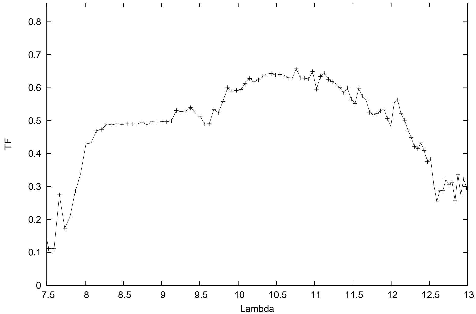
calHIP50371_flux-0.22962_diam5.18_r.MIDI.2012-02-24T05_50_51.000_D0H0
