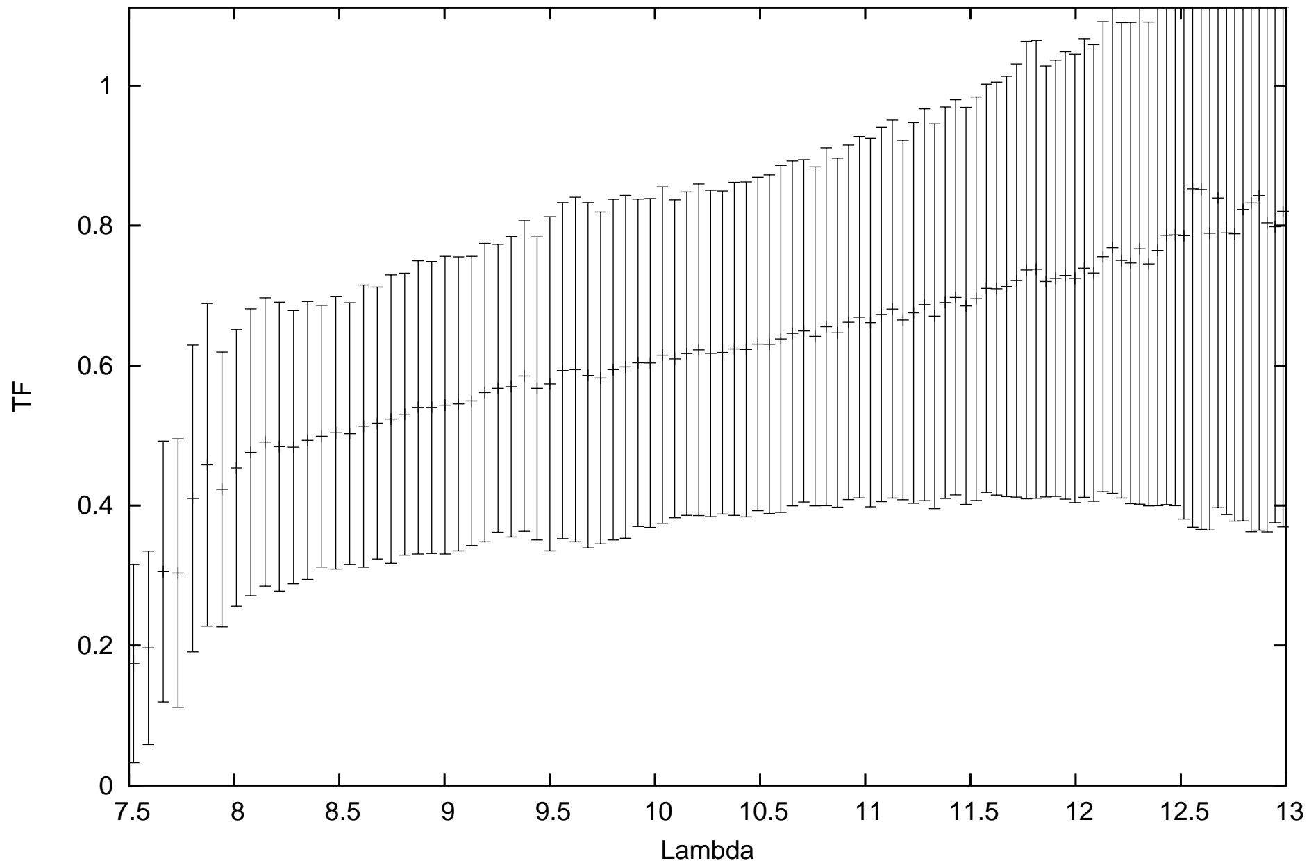
calHD108759_flux0.85_diam3.42_r.MIDI.2012-02-11T05_15_27.000_U3U4
