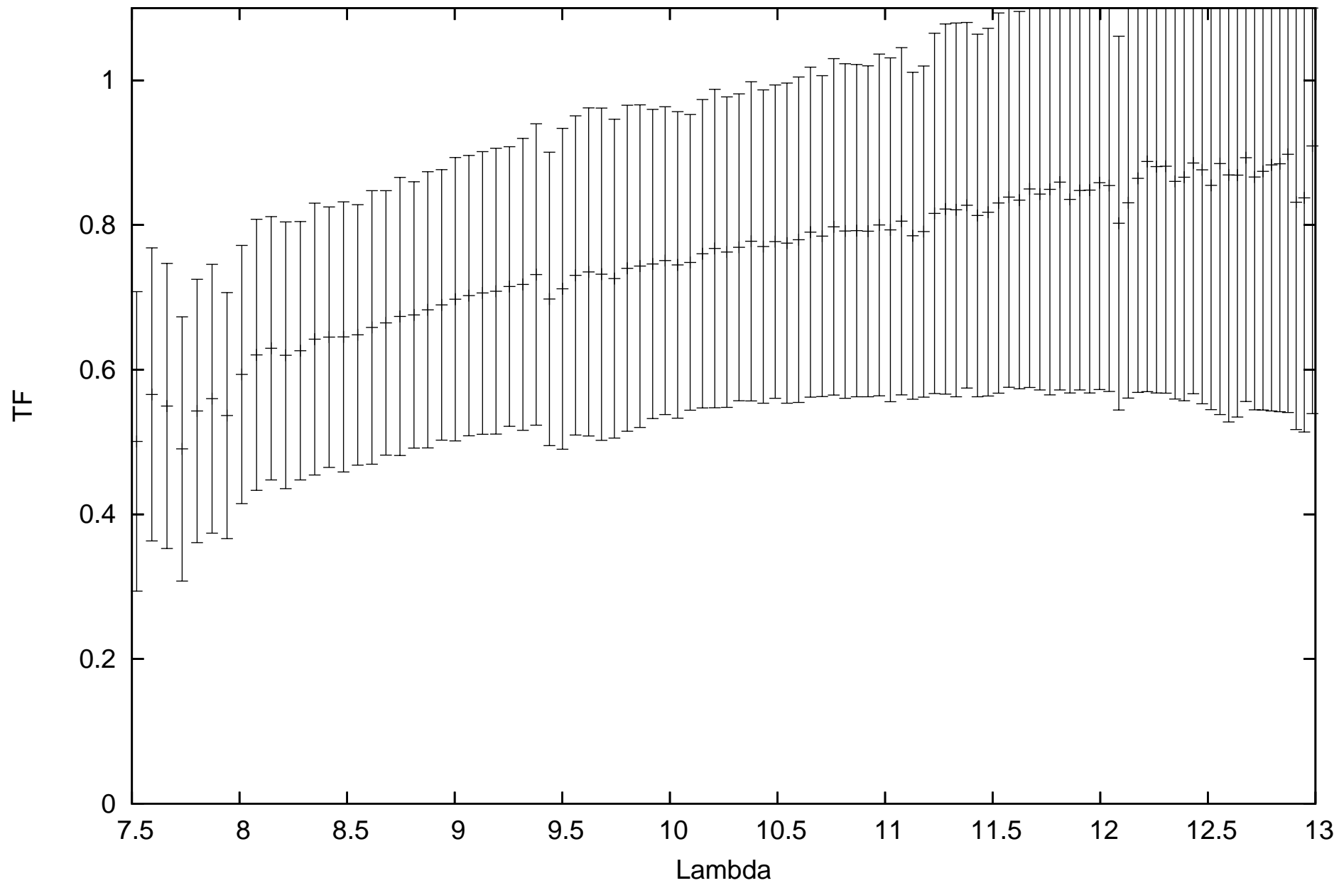
calHD108759_flux0.85_diam3.42_r.MIDI.2012-02-06T04_31_22.000_U1U2
