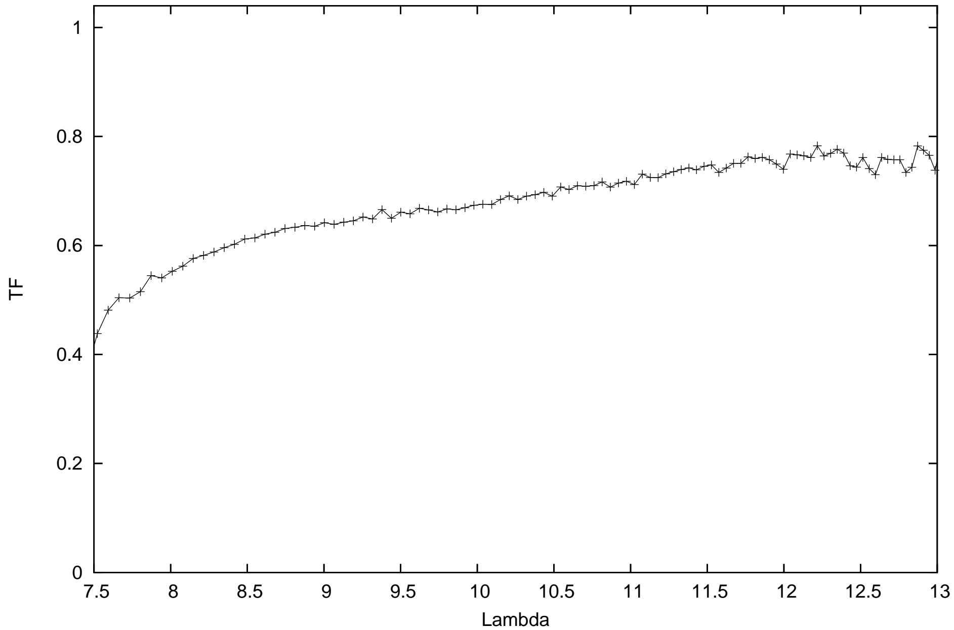
calHD63700_flux0.76_diam3.18_r.MIDI.2012-02-05T02_22_02.000_U3U4
