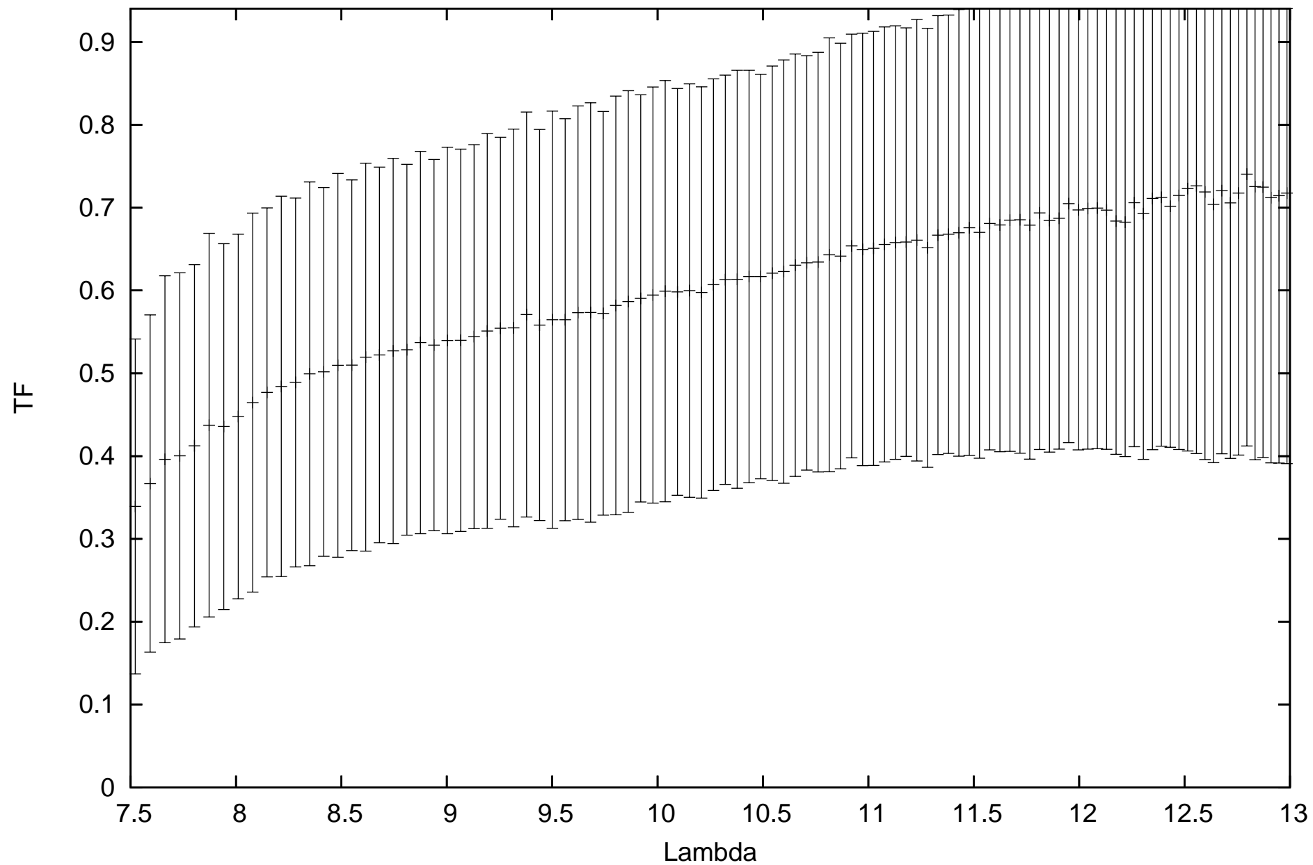
calHD63700_flux0.76_diam3.18_r.MIDI.2012-02-04T02_27_44.000_U2U3
