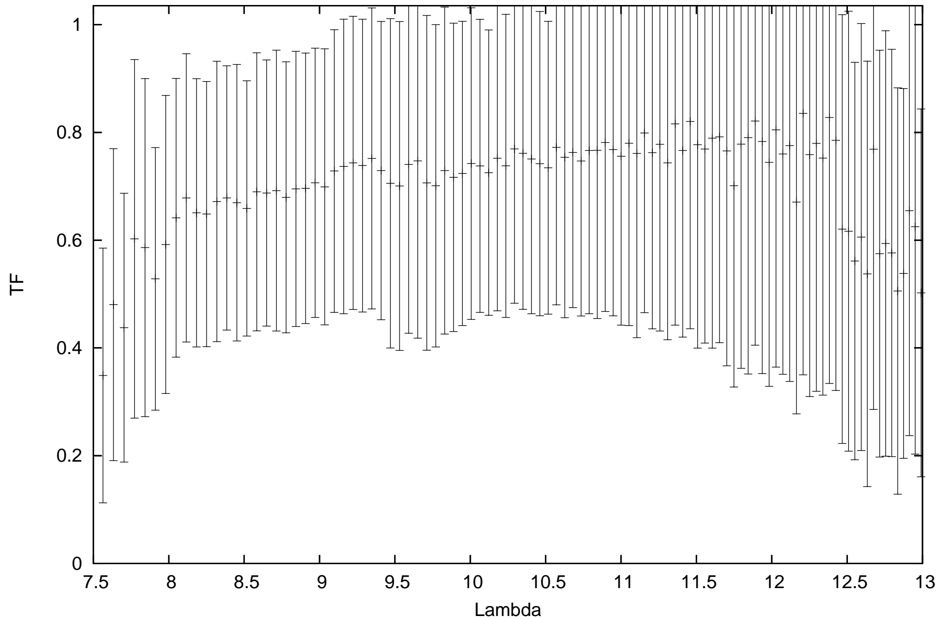
calHD81797_flux-1.49_diam9.14_r.MIDI.2012-02-01T07_40_45.970_B2A1
