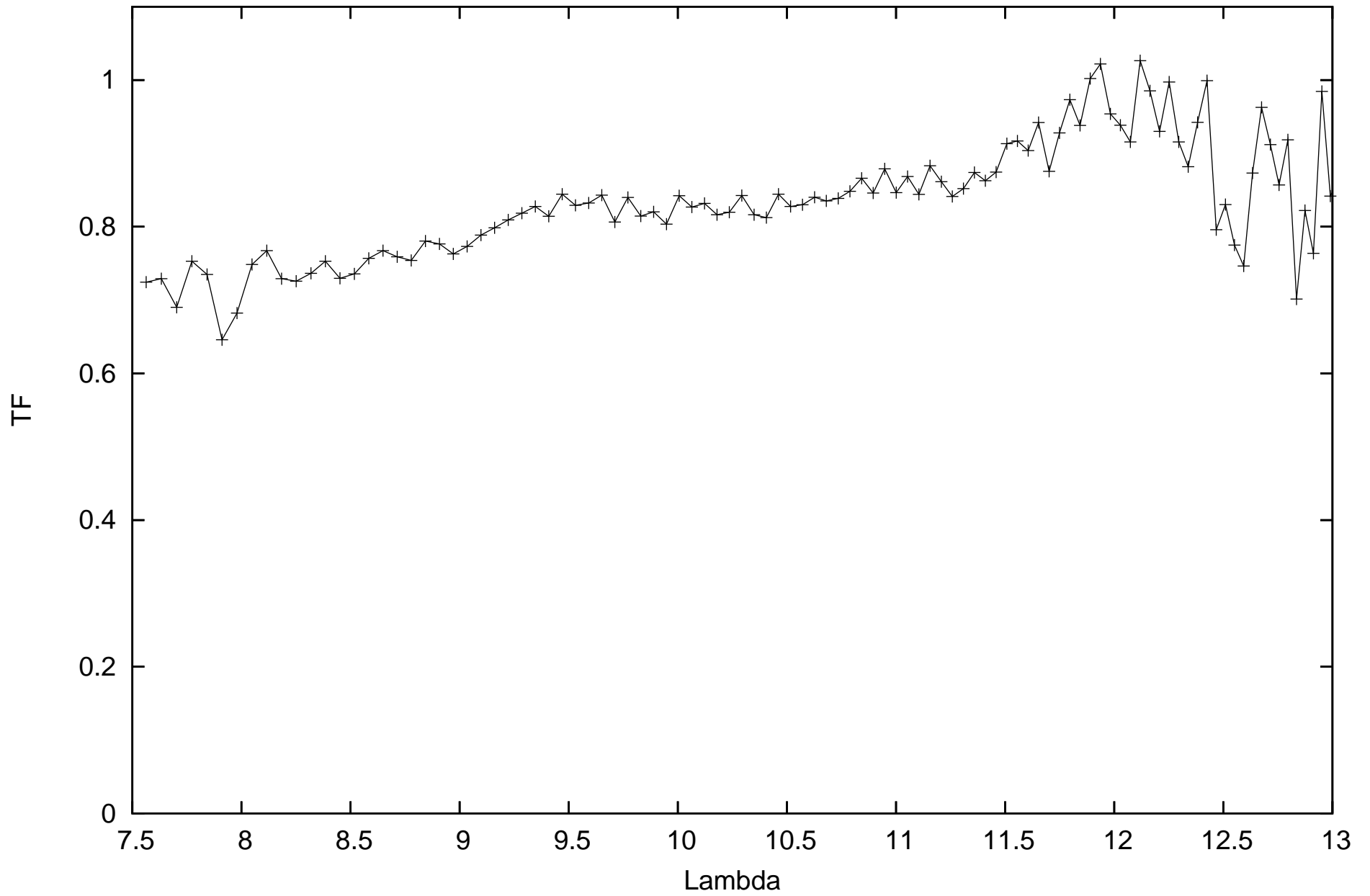
calHD81797_flux-1.49_diam9.14_r.MIDI.2012-02-01T07_12_33.105_C1B2
