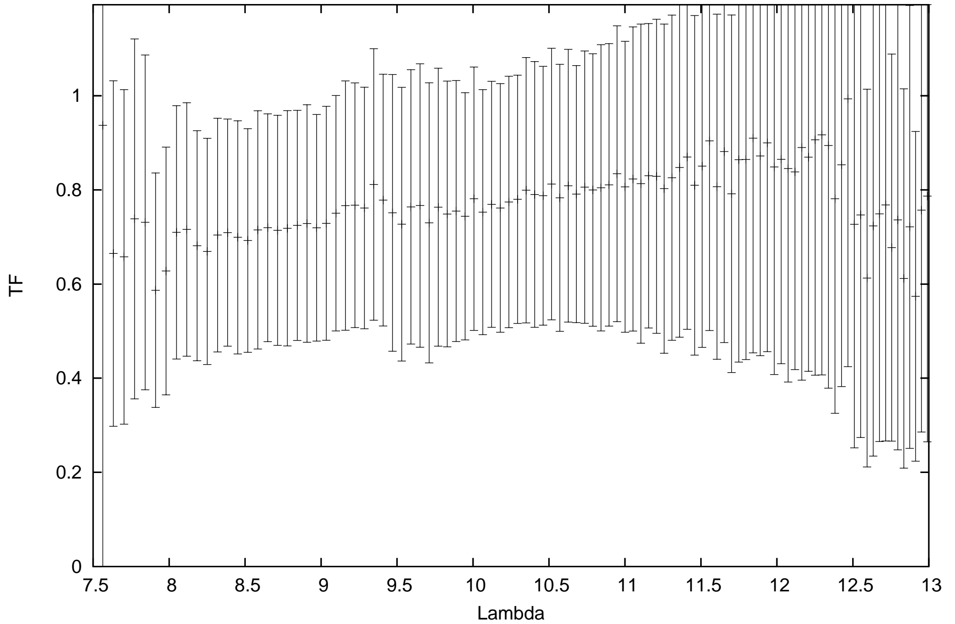
calHD81797_flux-1.49_diam9.14_r.MIDI.2012-02-01T06_18_44.293_C1B2
