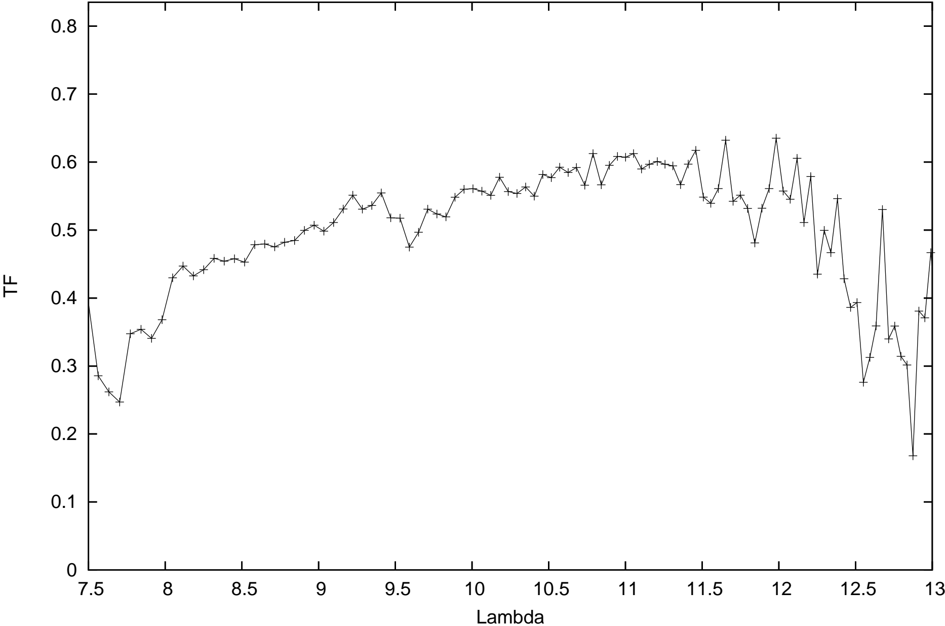
calHD81797_flux-1.49_diam9.14_r.MIDI.2012-02-01T05_30_36.135_B2A1
