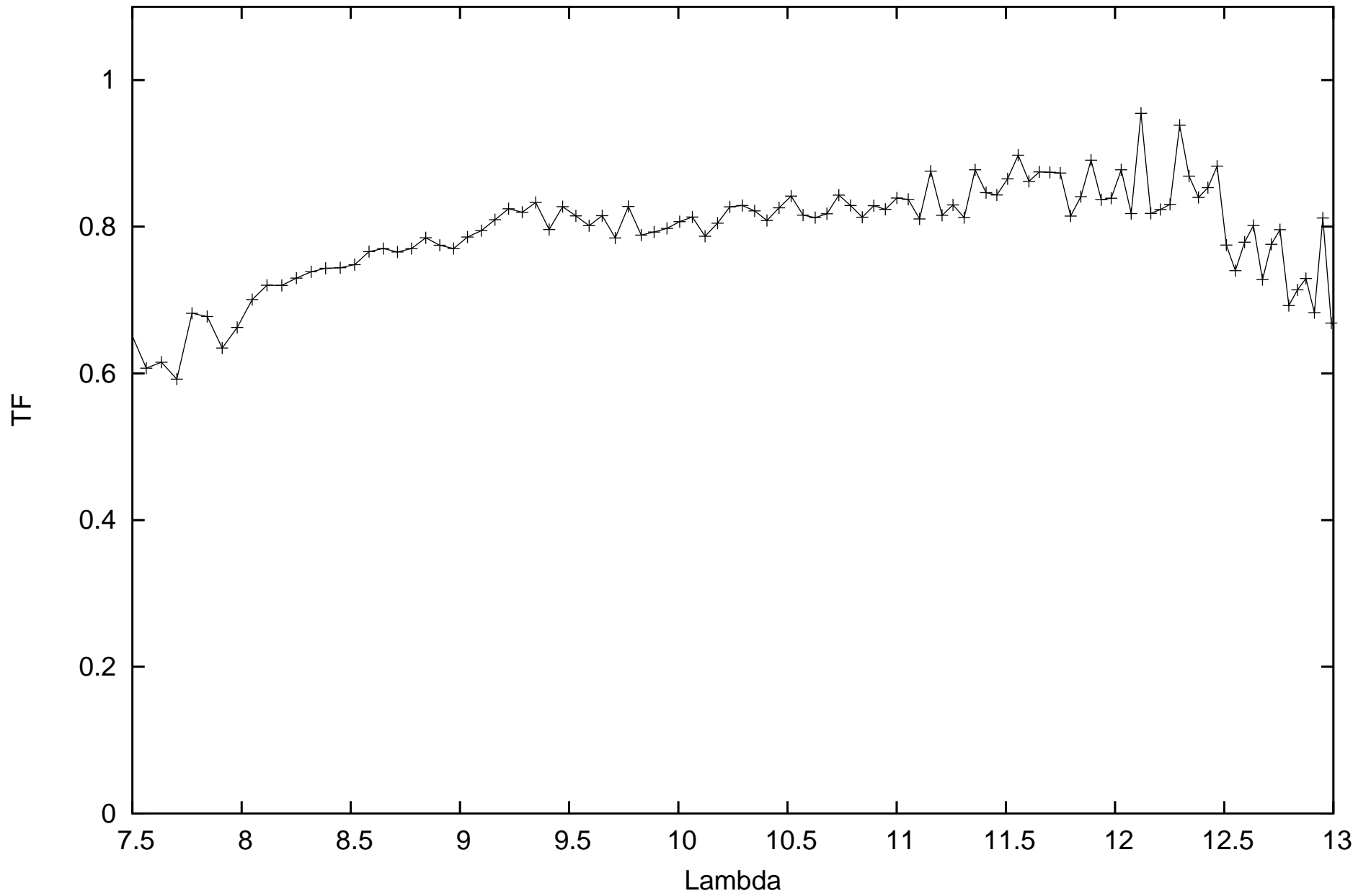
calHD81797_flux-1.49_diam9.14_r.MIDI.2012-01-24T06_39_37.135_C1A1
