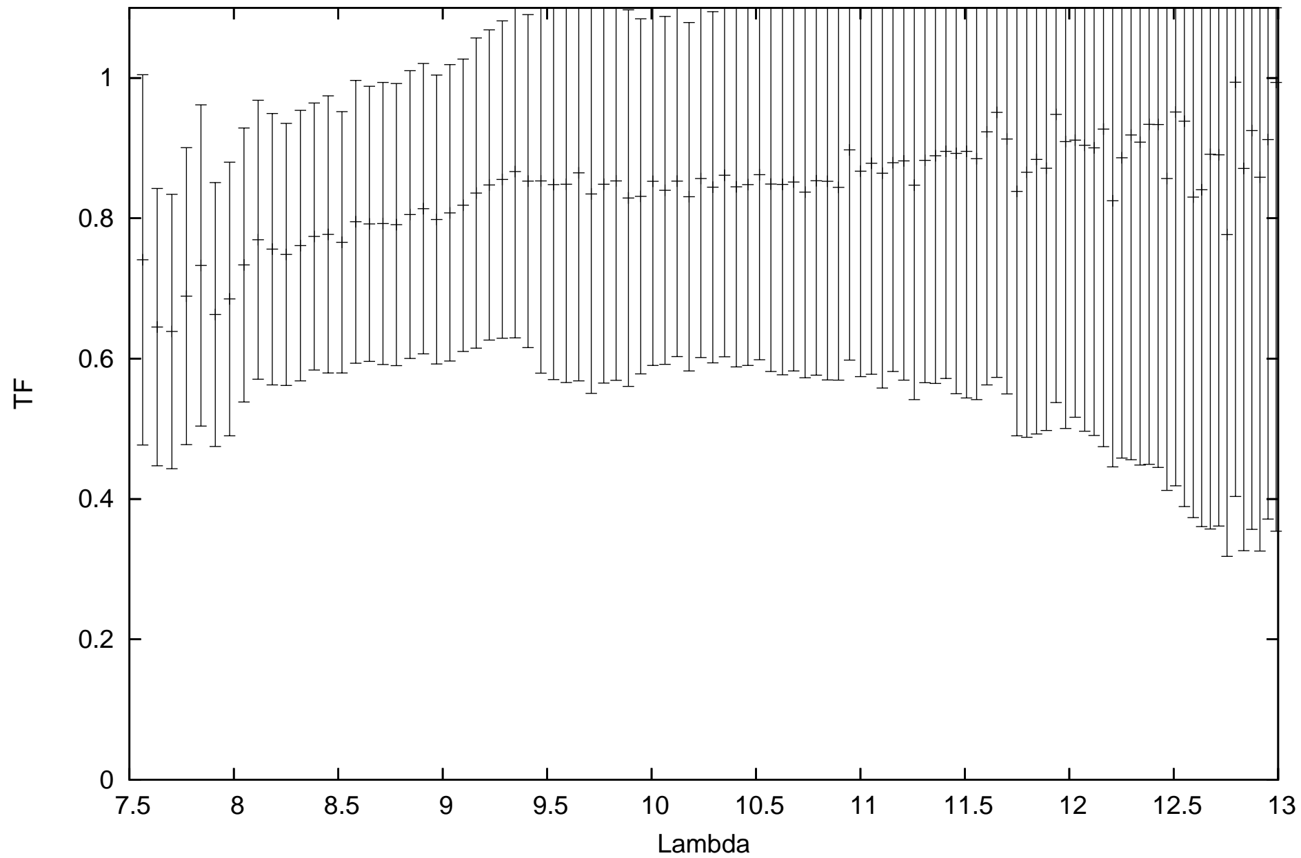
calHD81797_flux-1.49_diam9.14_r.MIDI.2012-01-24T04_29_13.970_C1A1
