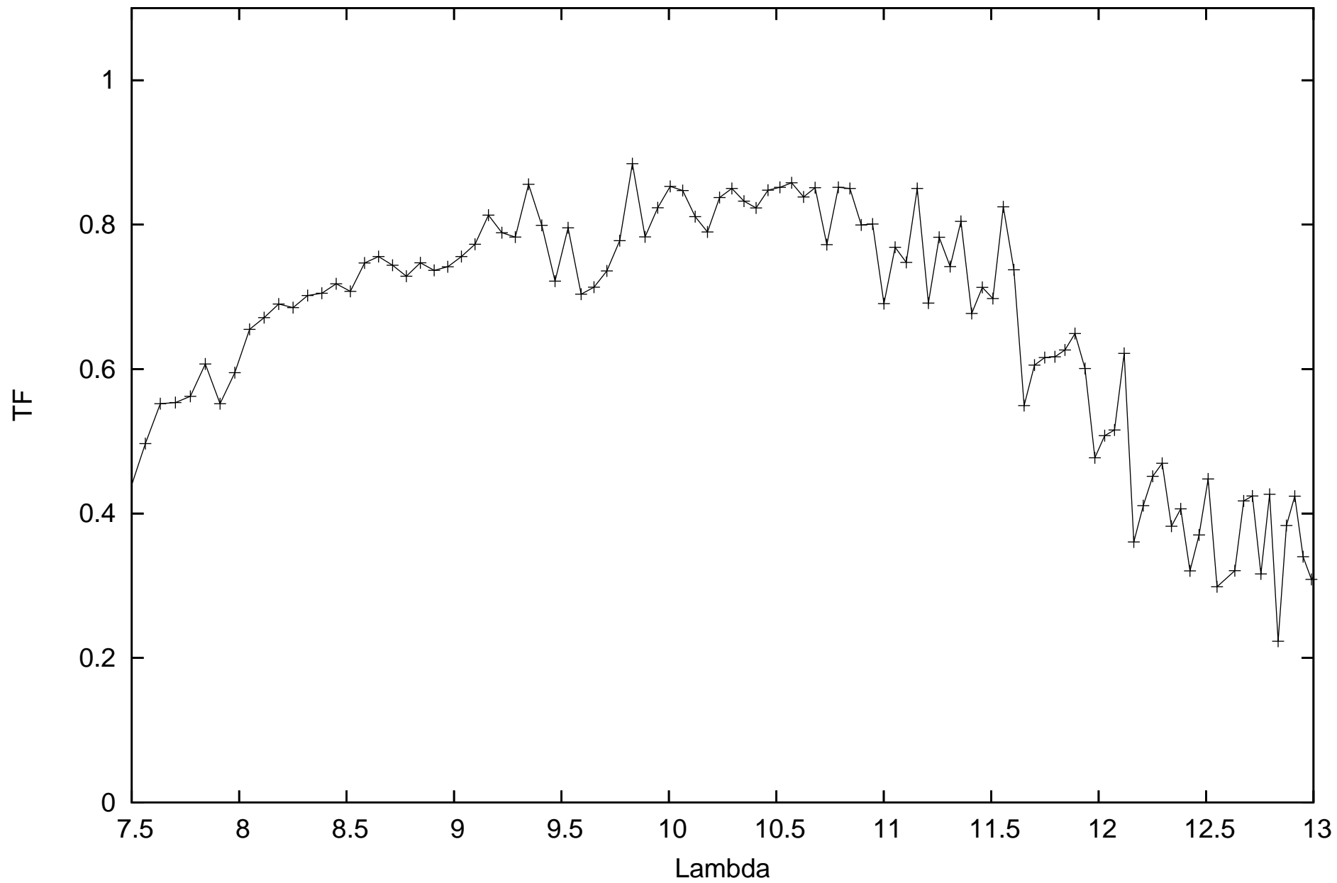
calHD123139_flux-0.39_diam5.34_r.MIDI.2012-01-24T08_56_14.969_C1A1
