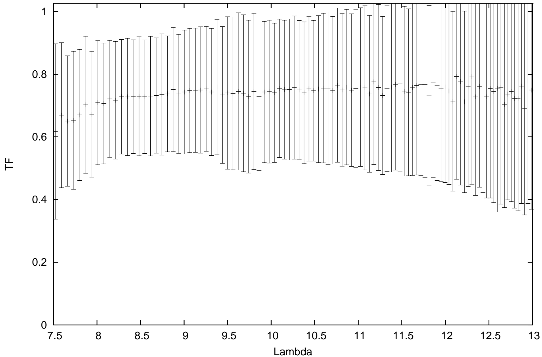
calHD20720_flux-1.53_diam10.14_r.MIDI.2012-01-22T02_00_47.000_D0A1
