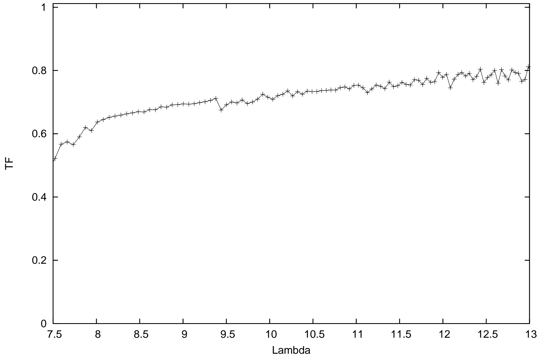
calHD29051_flux1.52_diam2.56_r.MIDI.2011-12-11T01_32_18.000_U2U3
